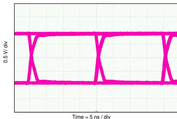
✎ 9-6. Eye Diagram at 50 Mbps PRBS 2^{16} - 1 , 1.8 V and 25°C
