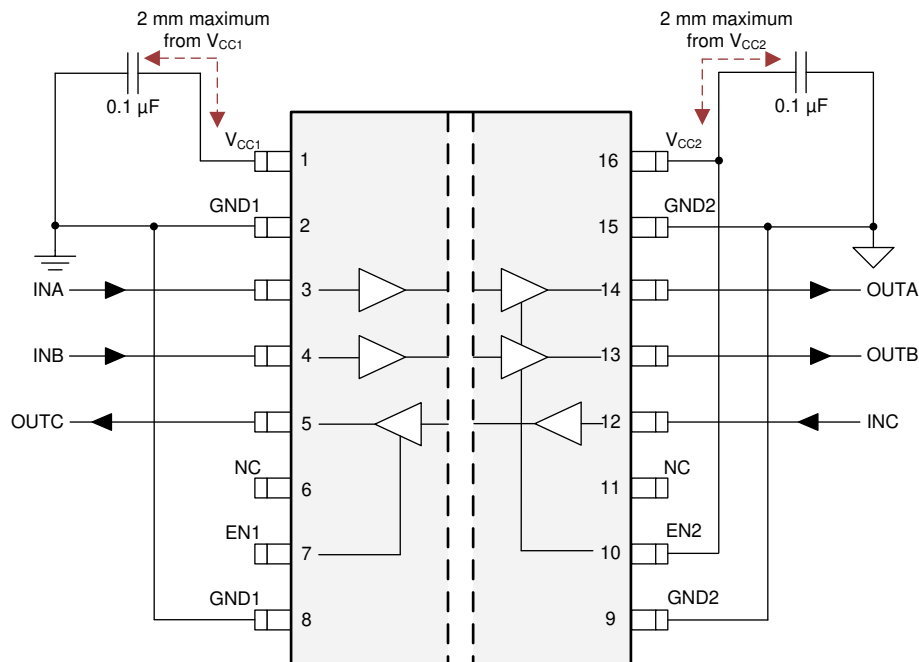
図 9-2. Typical ISO6731-Q1 Circuit Hook-up
