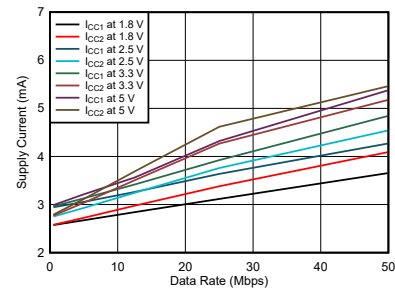
6-4. ISO6731-Q1 Supply Current vs Data Rate (With No Load)
