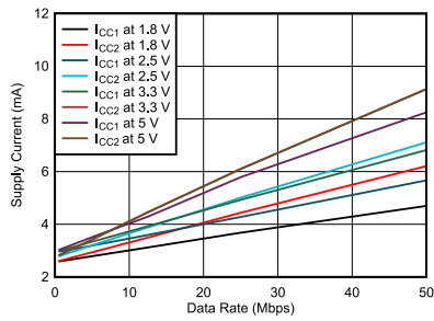
6-3. ISO6731-Q1 Supply Current vs Data Rate (With 15-pF Load)
