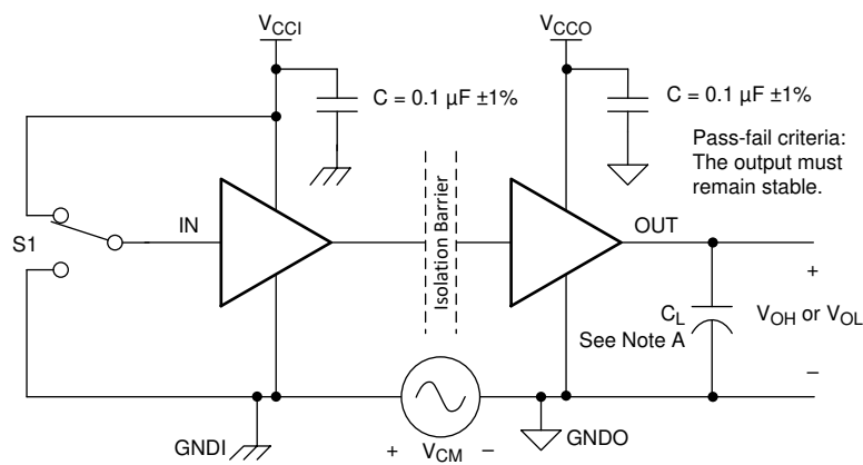
7-4. Common-Mode Transient Immunity Test Circuit
