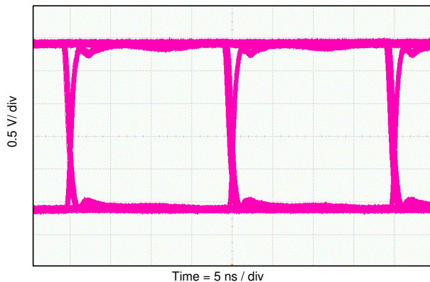
10-5. Eye Diagram at 50 Mbps PRBS 2^{16} - 1 , 2.5 V and 25°C
