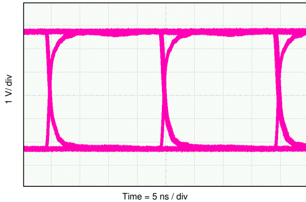
10-3. Eye Diagram at 50 Mbps PRBS 2^{16} - 1 , 5 V and 25°C
