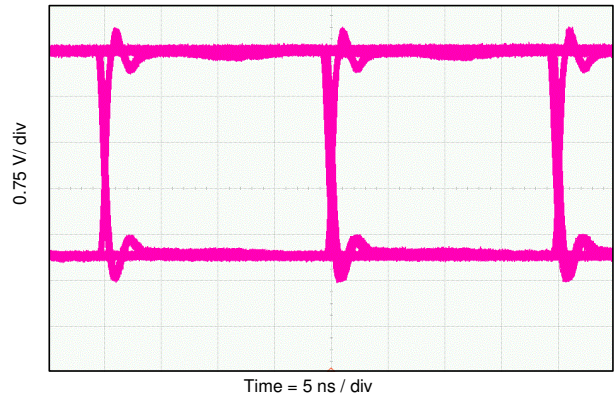
10-4. Eye Diagram at 50 Mbps PRBS 2^{16} - 1 , 3.3 V and 25°C
