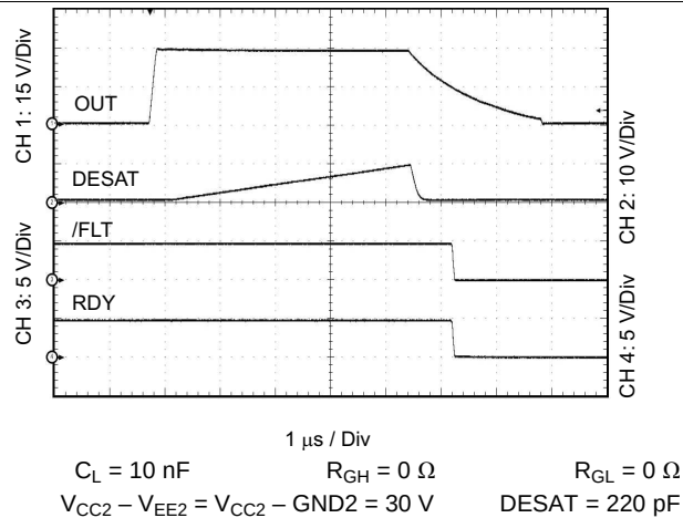
Figure 17. Output Transient Waveform DESAT, RDY, and FLT
