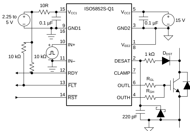
Figure 49. Unipolar Output Supply
