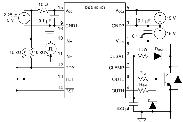
FIG 10-3. Bipolar Output Supply
