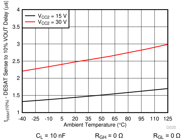
7-33. DESAT Sense to V_{OUT} 10% Delay vs Temperature
