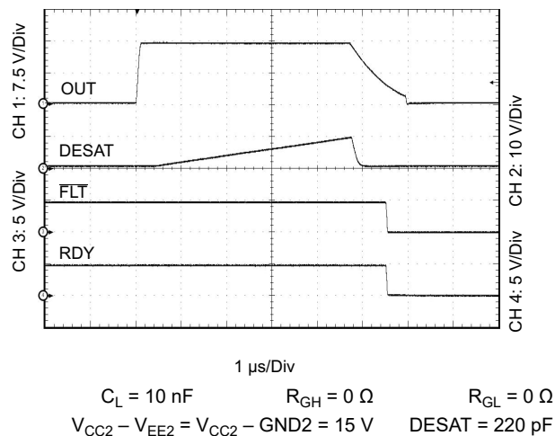
7-15. Output Transient Waveform DESAT, RDY, and \overline{\text{FLT}}
