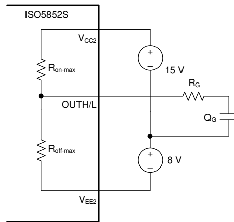
图 10-9. Simplified Output Model for Calculating P_{OL-WC}
