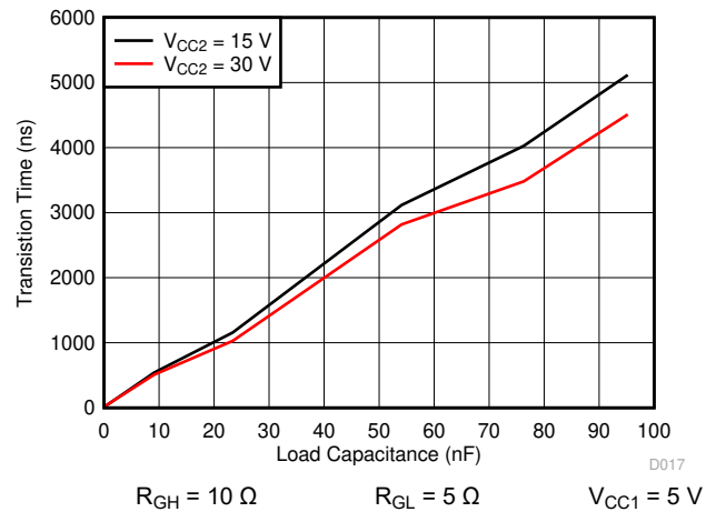
FIG 7-30. t_r Rise Time vs Load Capacitance
