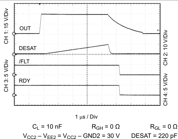
7-17. Output Transient Waveform DESAT, RDY, and \overline{\text{FLT}}
