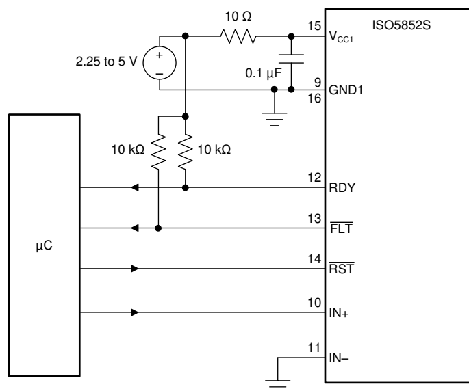
FIG 10-4. \overline{FLT} and RDY Pin Circuitry for High CMTI
