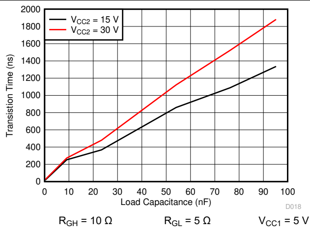
FIG 7-31. t_f Fall Time vs Load Capacitance
