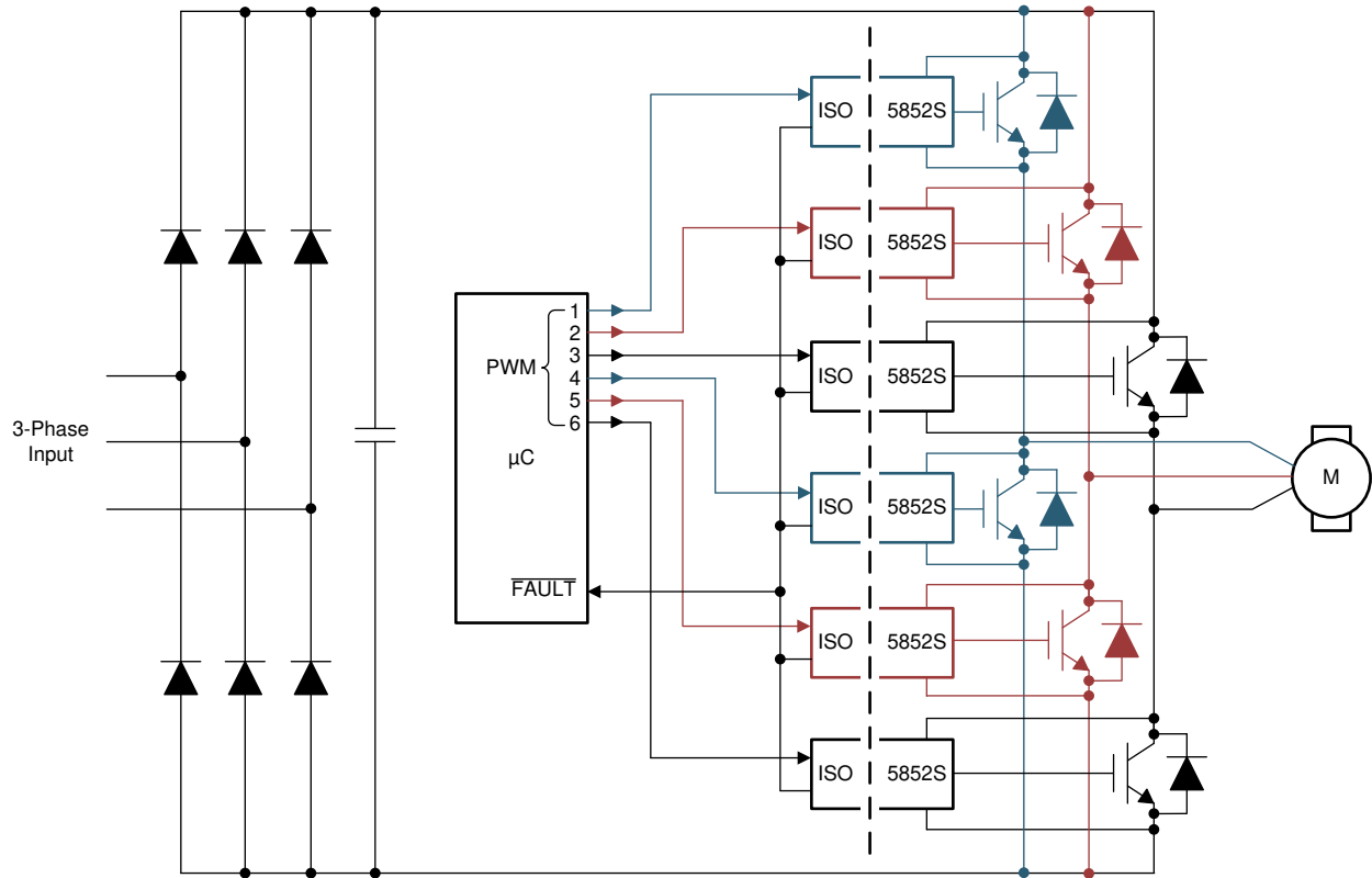
図 10-1. Typical Motor-Drive Application
