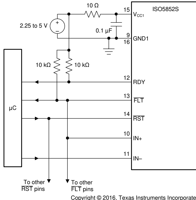
10-6. Global Shutdown With Inverting Input Configuration
