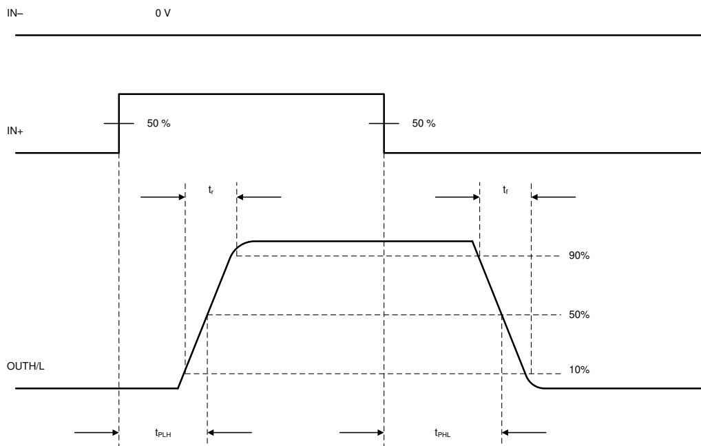
図 8-1. OUTH and OUTL Propagation Delay, Non-Inverting Configuration
