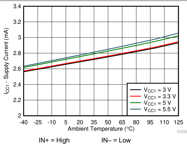
7-19. I_{CC1} Supply Current vs Temperature
