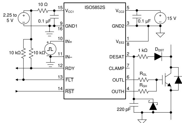
FIG 10-2. Unipolar Output Supply
