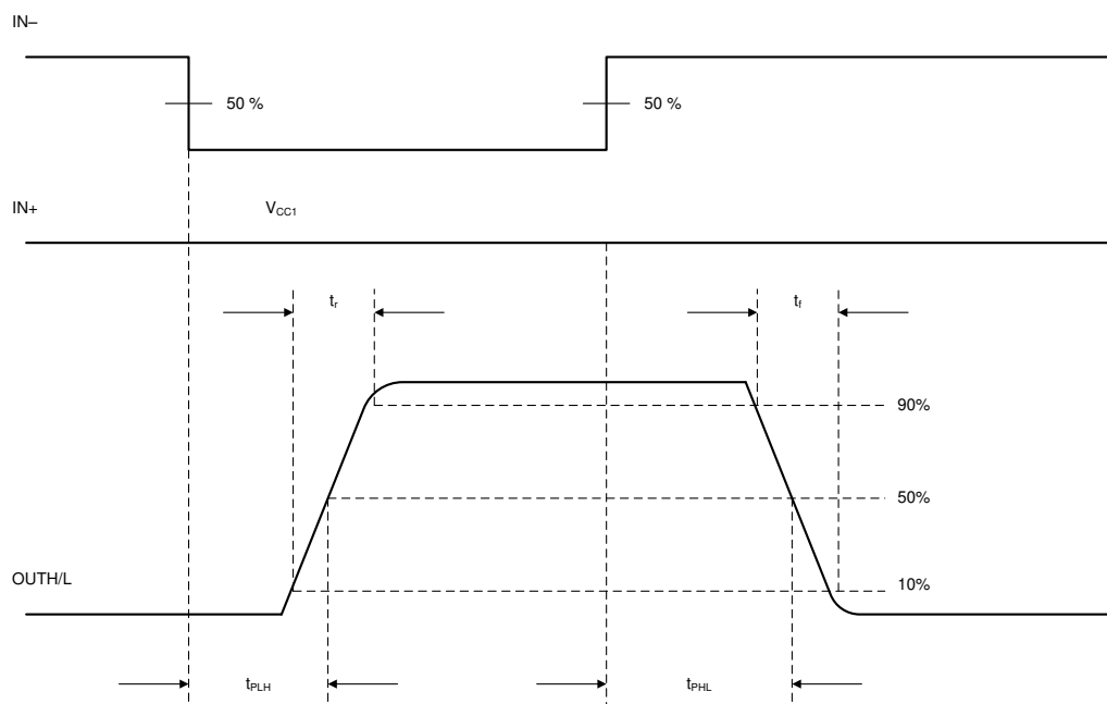
図 8-2. OUTH and OUTL Propagation Delay, Inverting Configuration
