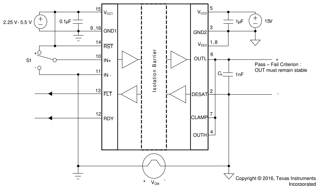
FIG 8-4. Common-Mode Transient Immunity Test Circuit
