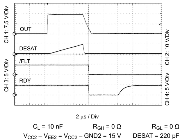
7-16. Output Transient Waveform DESAT, RDY, and \overline{\text{FLT}}
