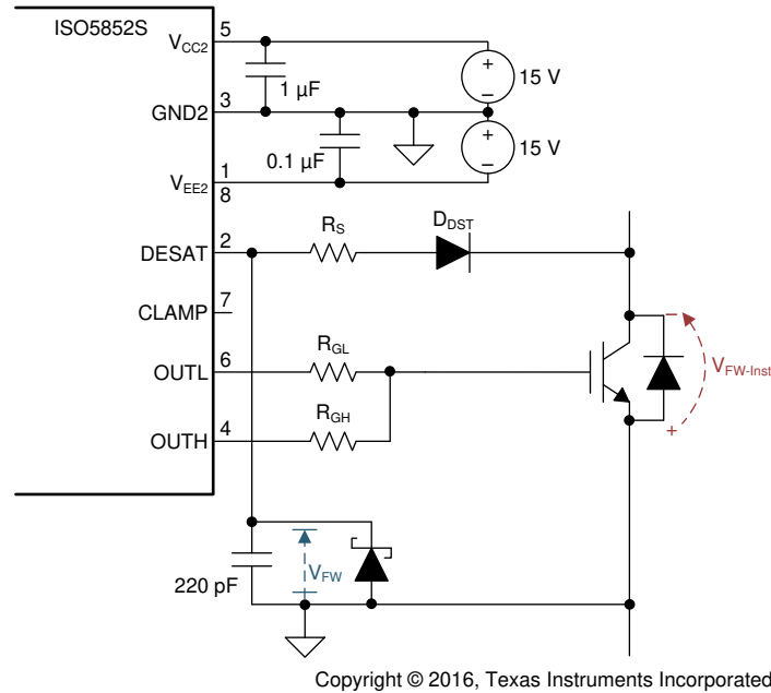
✎ 10-8. DESAT Pin Protection With Series Resistor and Schottky Diode
