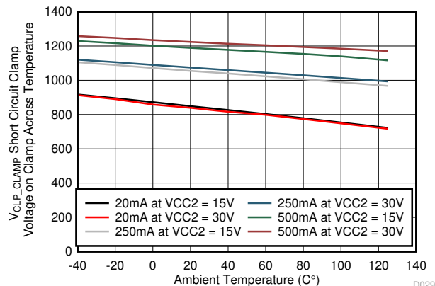
7-40. V_{CLP\_CLAMP} - Short-Circuit Clamp Voltage on CLAMP Across Temperature
