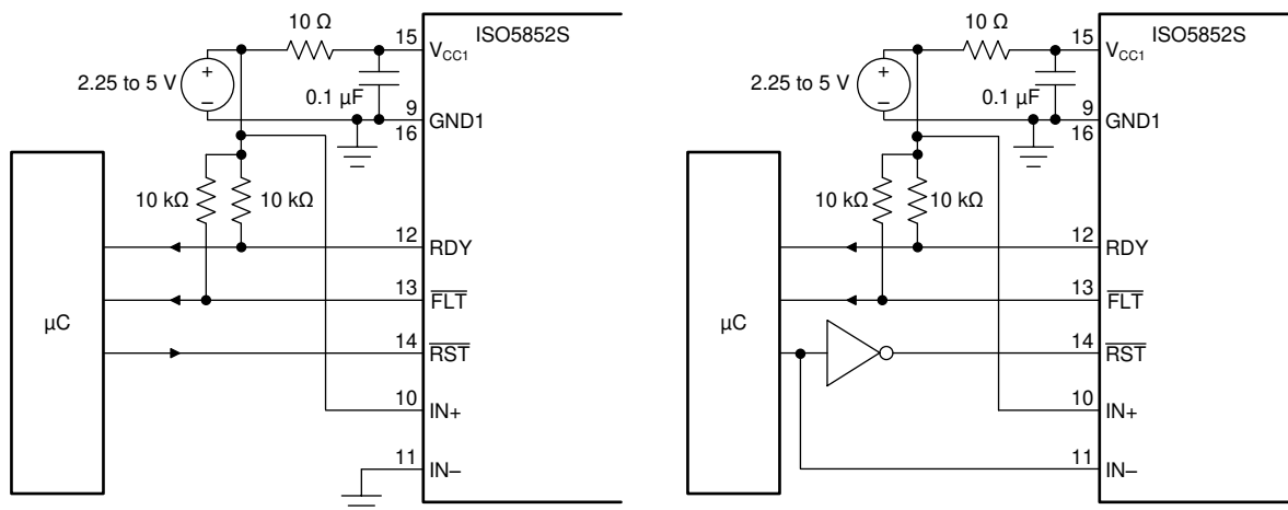
10-7. Auto Reset for Noninverting and Inverting Input Configuration
