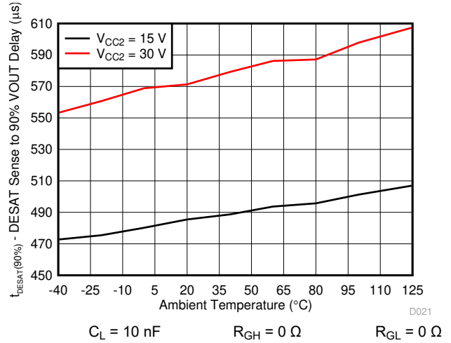
7-34. DESAT Sense to V_{OUT} 90% Delay vs Temperature
