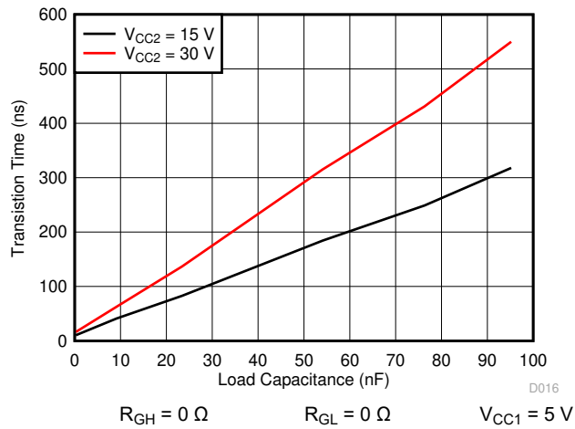
FIG 7-29. t_f Fall Time vs Load Capacitance
