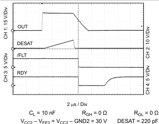
7-18. Output Transient Waveform DESAT, RDY, and \overline{\text{FLT}}
