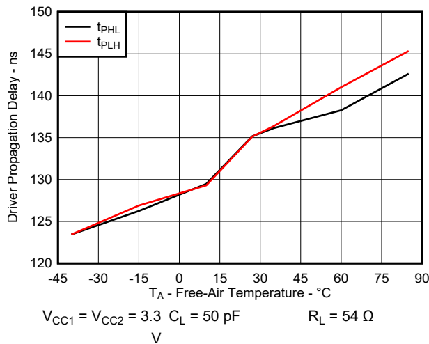
6-4. Driver Propagation Delay vs Free-Air Temperature
