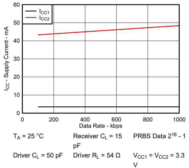
6-3. Supply Current vs Data Rate With Load
