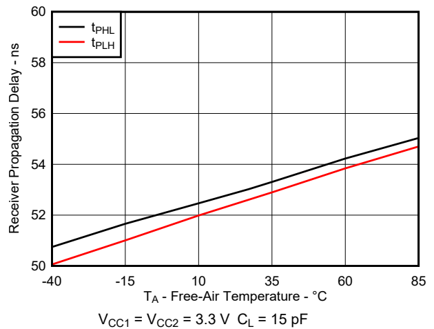
6-5. Receiver Propagation Delay vs Free-Air Temperature
