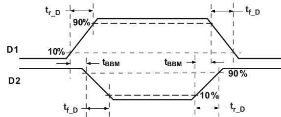
図 7-14. Transition Times and Break-Before-Make Time Delay for D1, D2 Outputs
