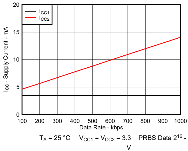
6-2. Supply Current vs Data Rate With No Load
