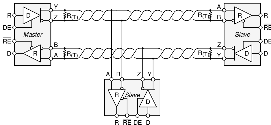
図 9-2. Typical RS-485 Network With Full-Duplex Transceivers
