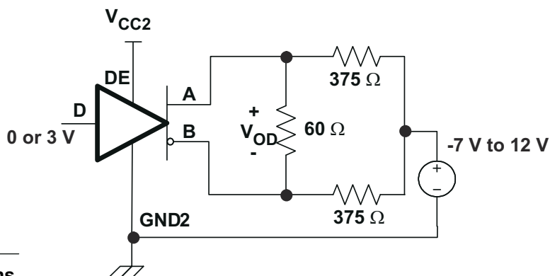
7-2. Driver V_{OD} With Common-Mode Loading Test Circuit
