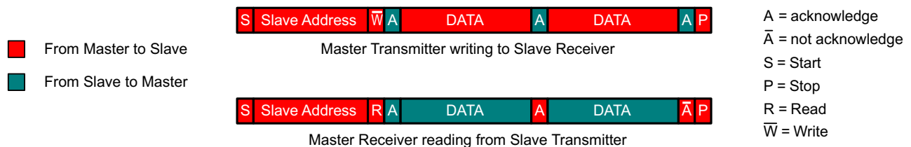
FIG 9-3. Transmit or Receive Mode Changes During a Data Transfer
