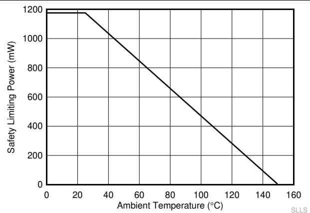
Figure 6-4. Thermal Derating Curve for Safety Limiting Power for DW-16 Package
