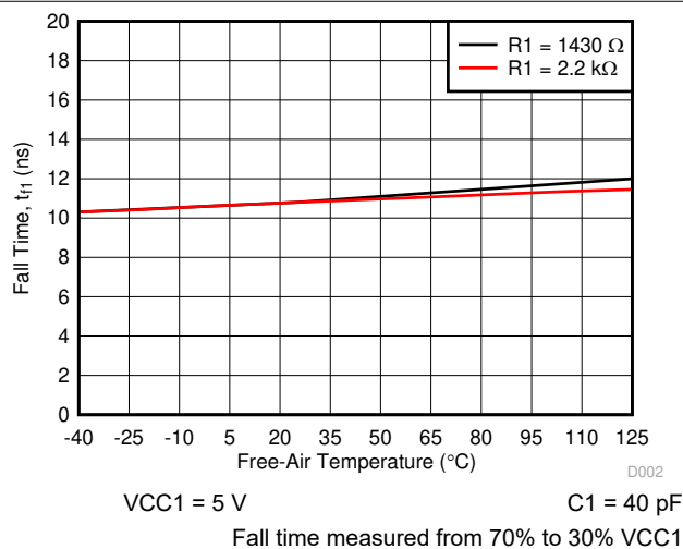
6-5. Side 1: Output Fall Time vs Free-air Temperature
