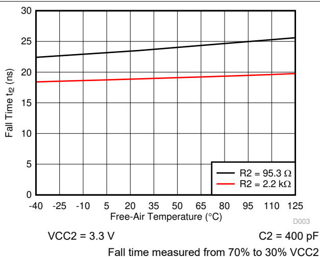
6-6. Side 2: Output Fall Time vs Free-Air Temperature
