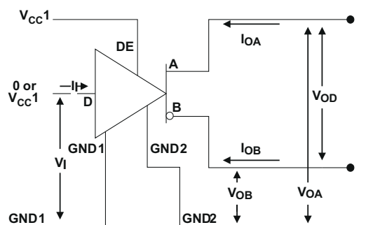
7-1. Open Circuit Voltage Test Circuit
