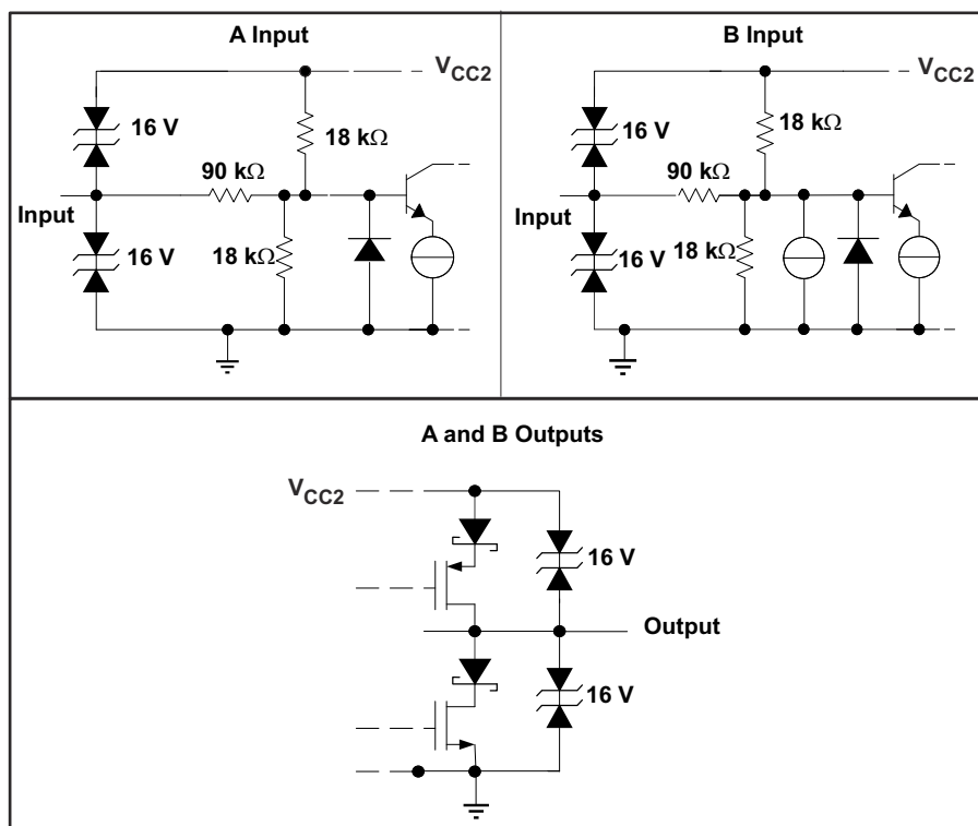
8-2. Equivalent I/O Schematics for A and B Inputs and Outputs
