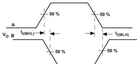
Figure 7-10. Driver Switching Test Circuit and Waveforms
