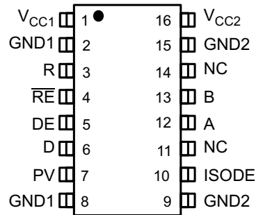
図 5-1. DW Package 16-Pin SOIC Top View
