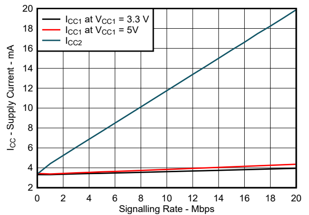
Figure 6-3. RMS Supply Current vs Signaling Rate
