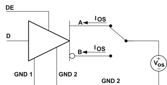
Figure 7-8. Driver Short-Circuit Test Circuit and Waveforms (Short-Circuit Applied at Time t=0 )
