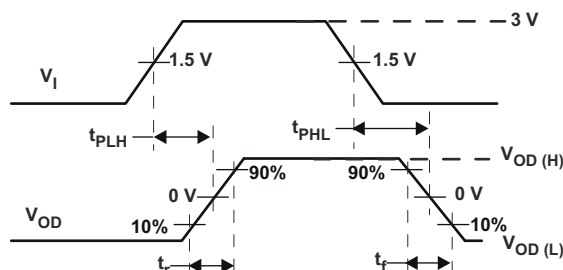
Figure 7-10. Driver Switching Test Circuit and Waveforms
