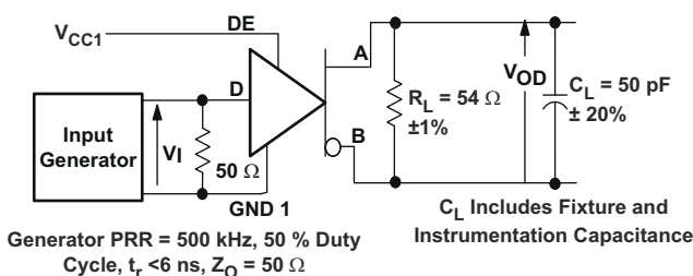
Figure 7-10. Driver Switching Test Circuit and Waveforms
