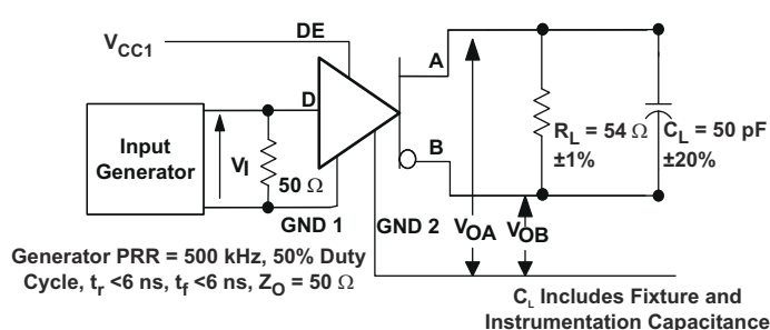
Figure 7-11. Driver Output Transition Skew Test Circuit and Waveforms
