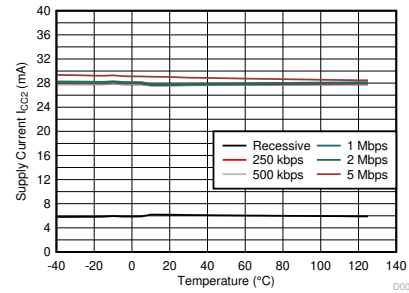
FIG 6-6. Side 2 Supply Current vs Ambient Temperature
