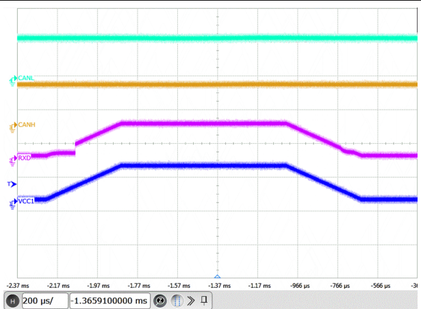
FIG 6-12. Glitch Free Power Up on VCC1 – CAN Bus Remains Recessive
