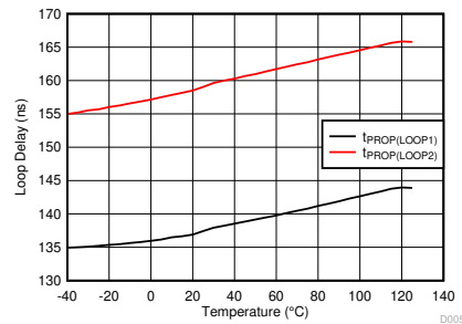
FIG 6-7. Loop Delay vs Ambient Temperature
