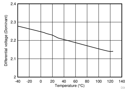
FIG 6-8. Dominant state differential output voltage vs Ambient Temperature
