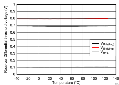
FIG 6-10. Receiver differential threshold voltage vs Ambient Temperature
