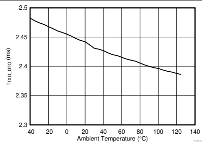
FIG 6-11. Dominant timeout vs Ambient Temperature
