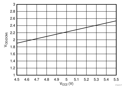
FIG 6-9. Dominant state differential output voltage vs Side2 supply voltage
