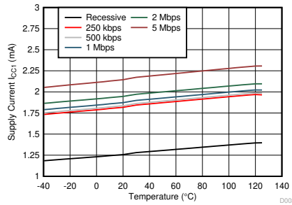
FIG 6-5. Side 1 Supply Current vs Ambient Temperature
