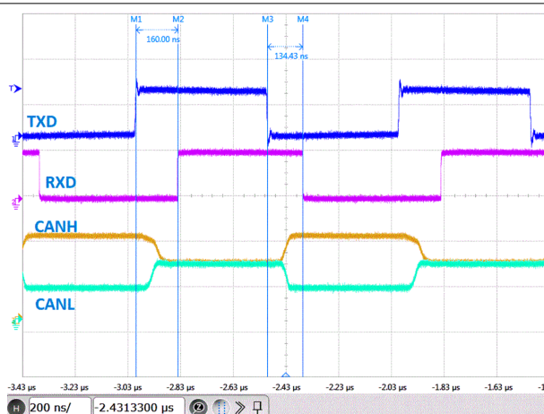
图 6-14. Typical TXD, RXD, CANH and CANL Waveforms at 2 Mbps
