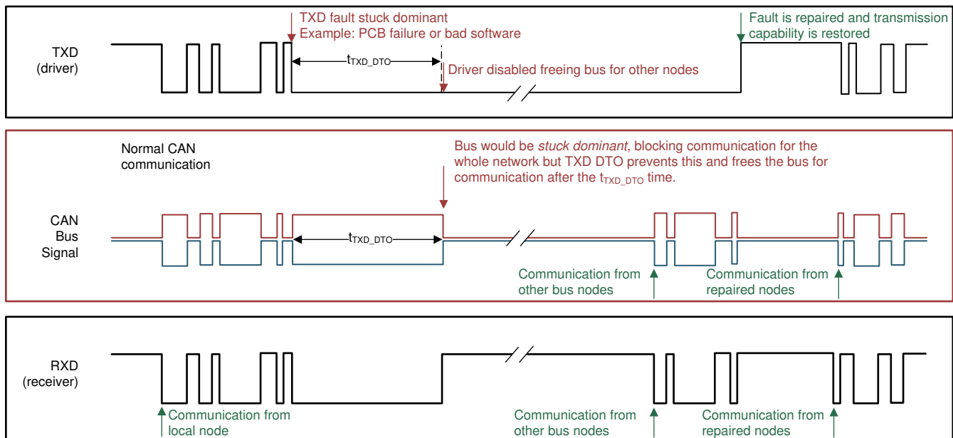
図 27. Example Timing Diagram for TXD DTO
