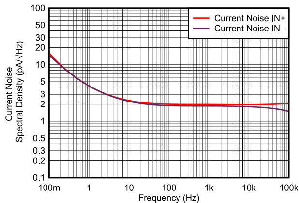
7-19. Current Noise Spectral Density vs Frequency (RTI)
