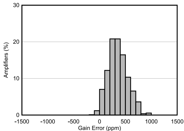
7-7. Typical Distribution of Gain Error
