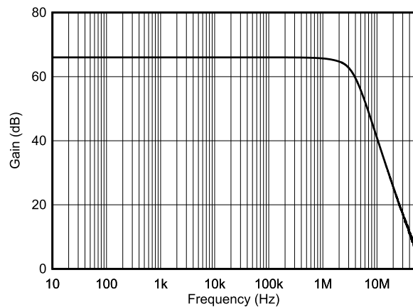
7-22. Closed Loop Gain vs Frequency
