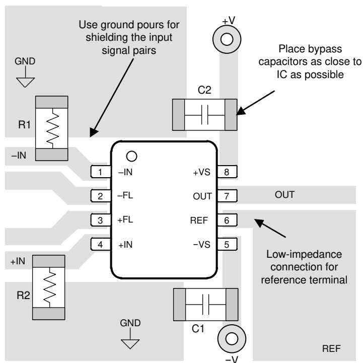
11-1. Example Schematic and Associated PCB Layout (inductors and capacitors shown on FL pins are optional)
