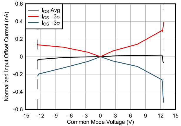
7-14. Input Offset Current vs Input Common-Mode Voltage
