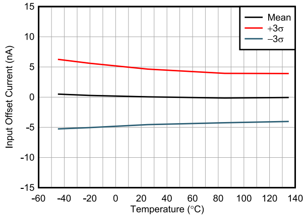
7-13. Input Offset Current vs Temperature
