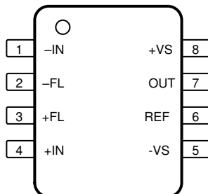
6-1. D Package, 8-Pin SOIC, Top View
