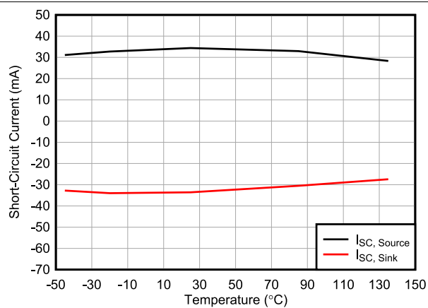
7-31. Short Circuit Current (Source + Sink) vs Temperature
