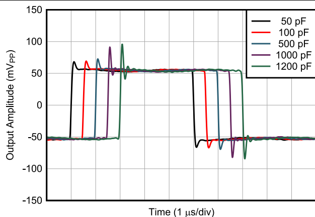
7-25. Small Signal Response
