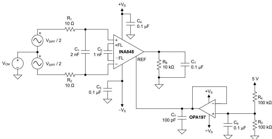
Figure 9-4. Sensor Conditioning ( V_{DIFF} < 5 \text{ mV} , V_{S\pm} = 15 \text{ V} )
