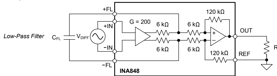
図 9-1. Low-pass Filter
