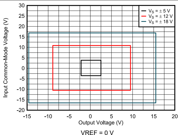
7-9. Input Common-Mode Voltage vs Output Voltage
