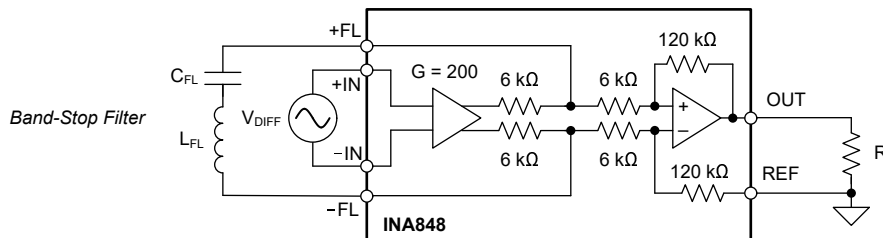
図 9-2. Bandstop Filter
