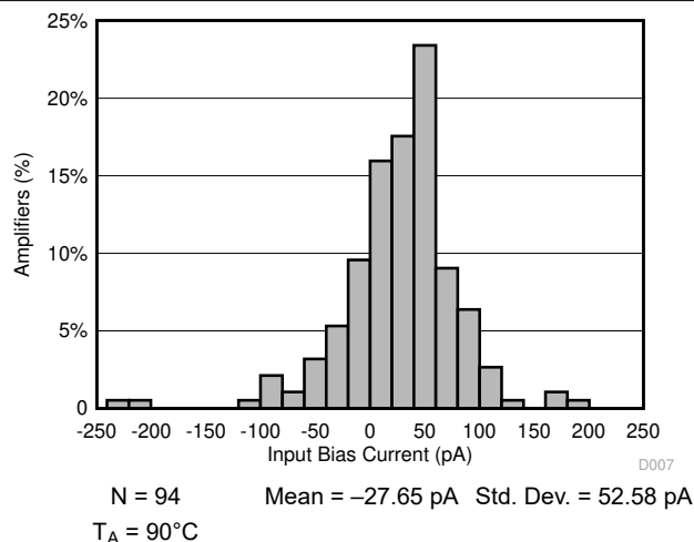
7-8. Typical Distribution of Input Bias Current
