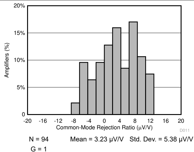
7-12. Typical CMRR Distribution
