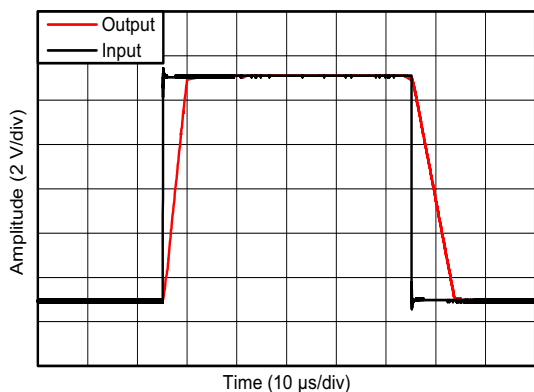
FIG 45. Small-Signal Response
