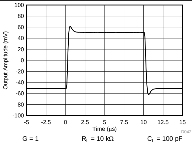
FIG 43. Small-Signal Response
