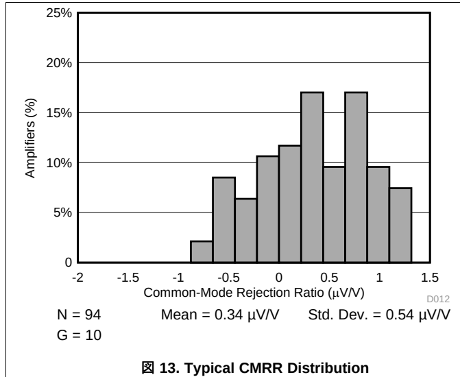
Figure 13. Typical CMRR Distribution
