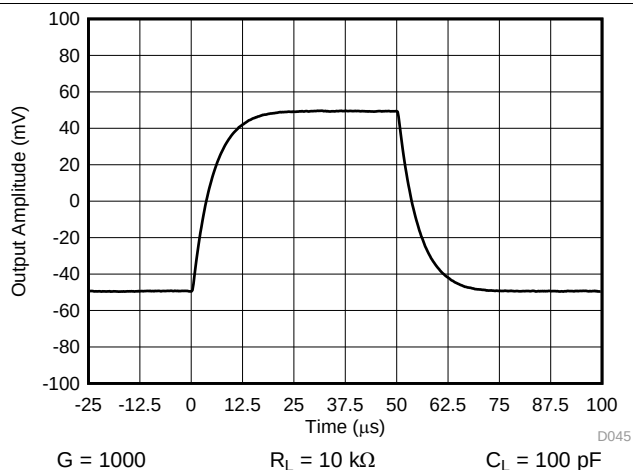
FIG 46. Small-Signal Response
