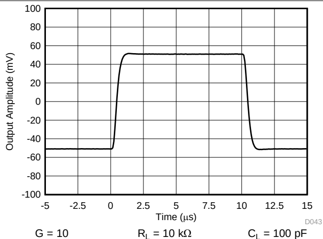
FIG 44. Small-Signal Response
