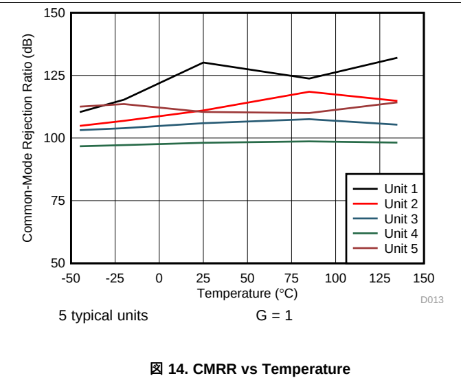
Figure 14. CMRR vs Temperature
