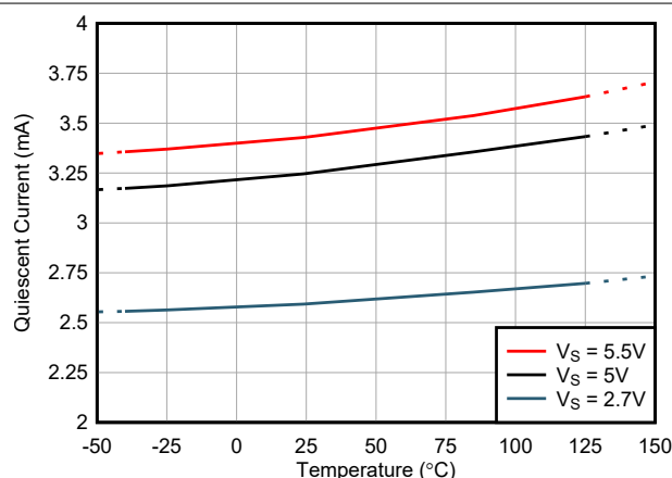
图 5-23. Quiescent Current vs Temperature
