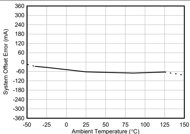
FIG 5-2. INA790B Input Offset Current vs Temperature
