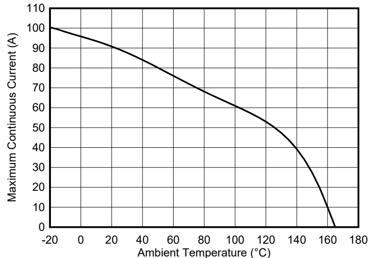
FIG 6-2. Maximum Continuous Current vs Ambient Temperature
