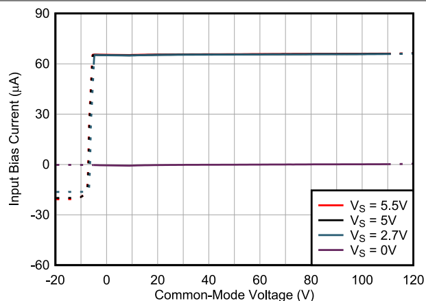
图 5-20. Total Input Bias Current vs Common-Mode Voltage
