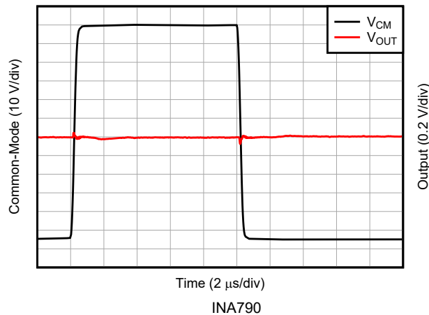
図 5-29. -4V to 110V Common-Mode Step Transient Response
