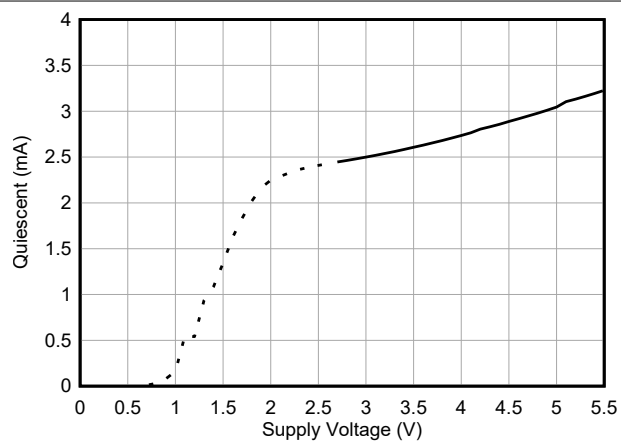
图 5-22. Quiescent Current vs Supply Voltage
