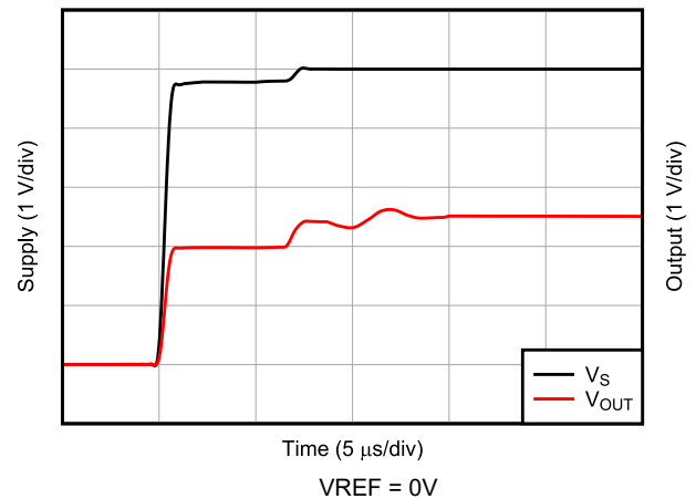
図 5-30. Start-Up Response
