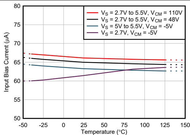
图 5-21. Total Input Bias Current vs Temperature
