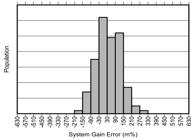
FIG 5-7. INA790B Gain Error Production Distribution
