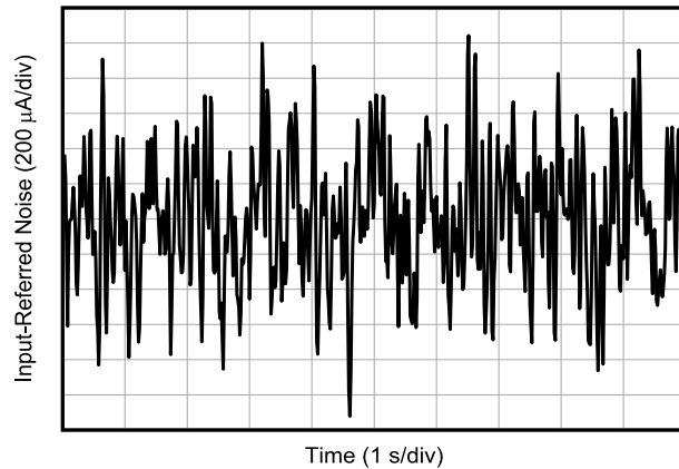
図 5-27. 0.1Hz to 10Hz Input-Referred Current Noise
