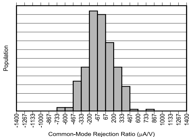
FIG 5-3. INA790B Common-Mode Rejection Production Distribution
