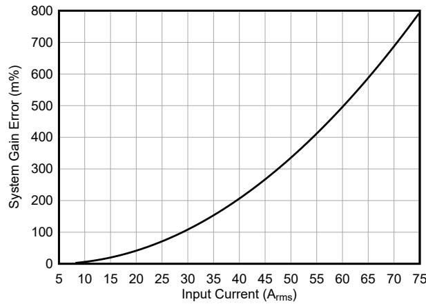
FIG 5-9. INA790B System Gain Error vs Input Current
