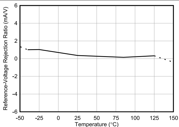
FIG 5-6. Reference Voltage Rejection Ratio vs Temperature
