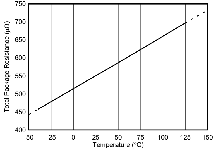
FIG 6-1. IS+ to IS– Package Resistance vs Temperature
