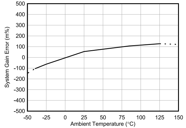
FIG 5-8. INA790B Gain Error vs Temperature
