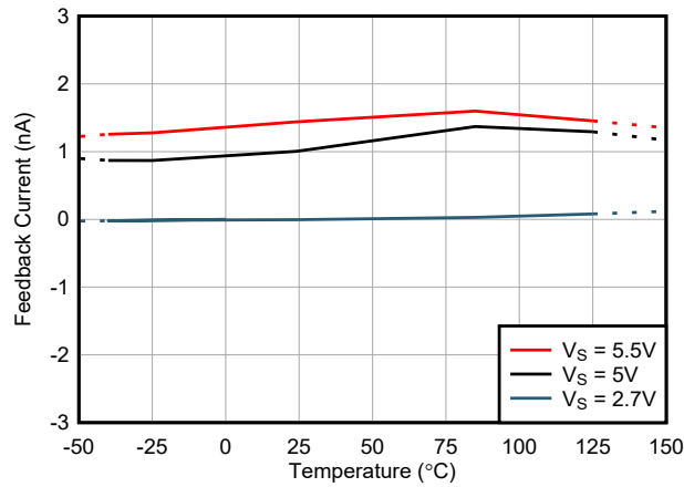
図 5-25. Feedback Current vs Temperature
