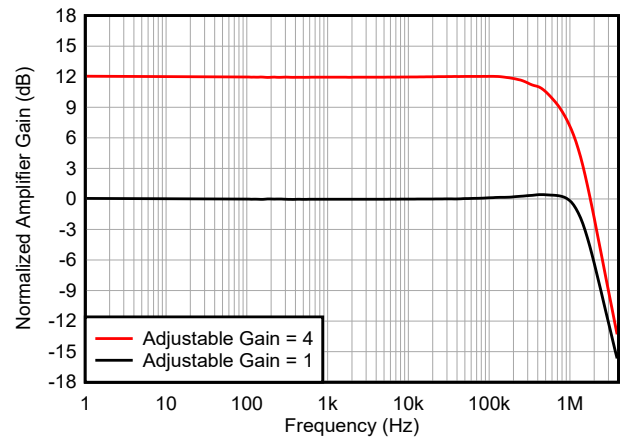
FIG 5-10. Current Sense Amplifier Gain vs Frequency
