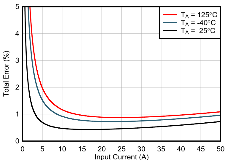
図 7-1. INA790A Total Error vs Input Current
