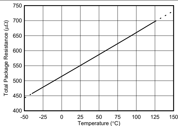
图 5-19. Package Resistance vs Temperature
