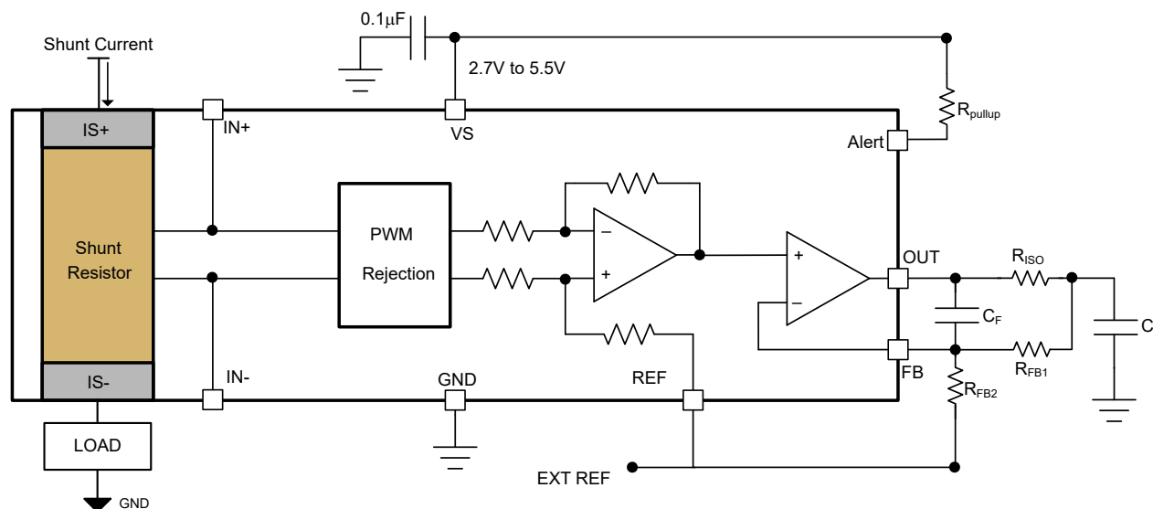
図 7-5. INA790x With RISO-Dual-Feedback
