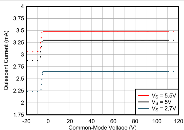
图 5-24. Quiescent Current vs Common-Mode Voltage
