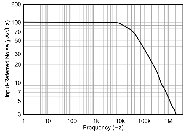
図 5-26. INA790A Input-Referred Current Noise vs Frequency
