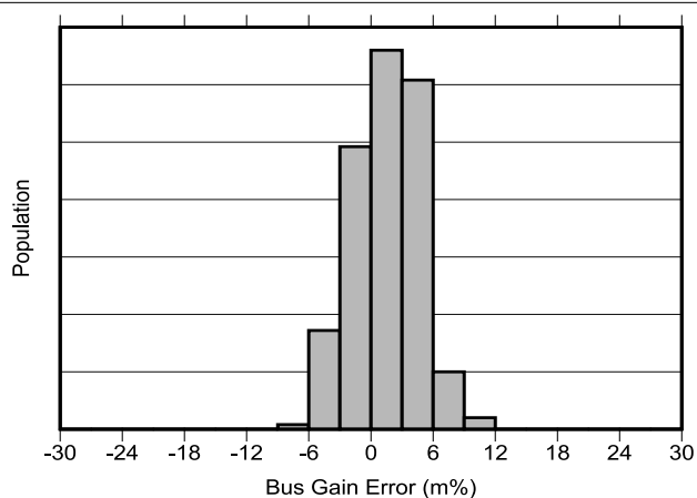
5-11. Bus Input Gain Error Production Distribution
