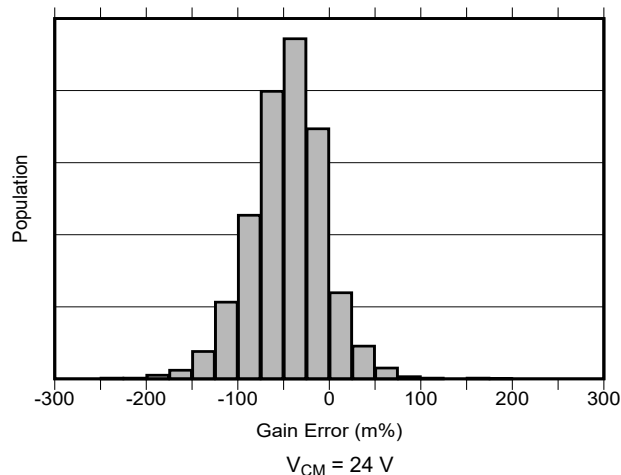
FIG 5-6. Current Gain Error Production Distribution
