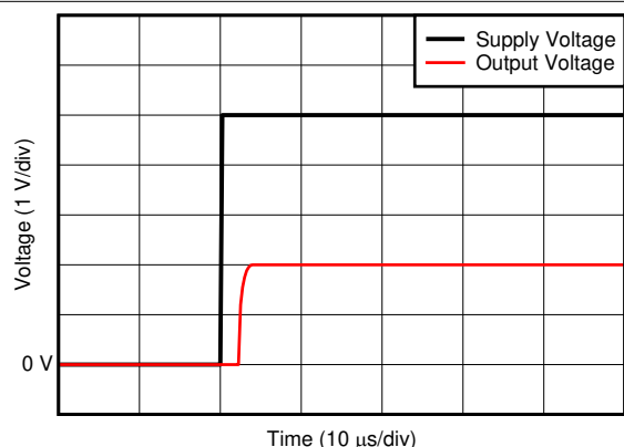
7-35. Start-Up Response
