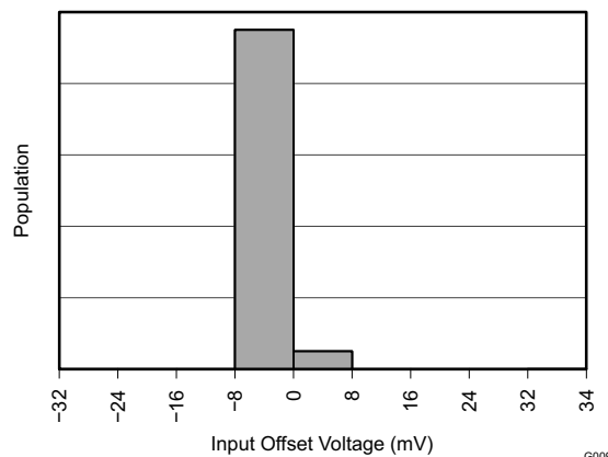
FIG 7-8. Bus Input Offset Voltage Production Distribution
