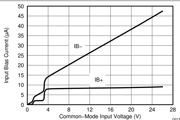
FIG 7-12. Input Bias Current vs. Common-Mode Voltage
