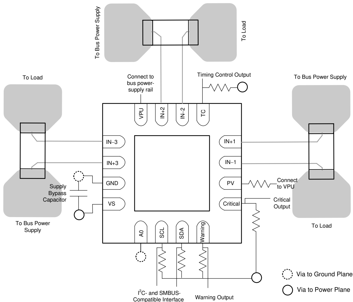
11-1. Layout Example
