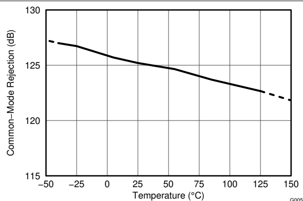
7-4. Shunt Input Common-Mode Rejection Ratio vs. Temperature
