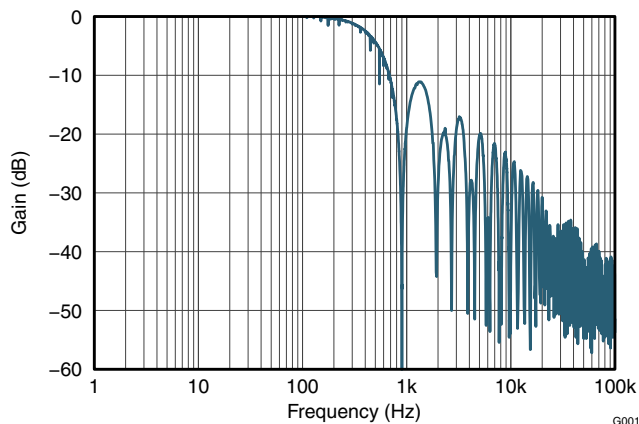
7-1. Frequency Response
