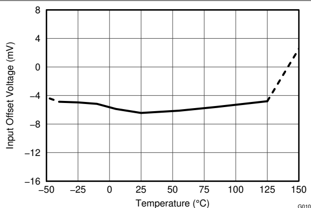
FIG 7-9. Bus Input Offset Voltage vs. Temperature
