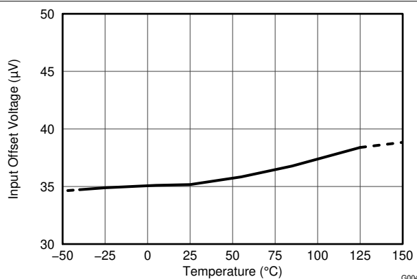
7-3. Shunt Input Offset Voltage vs. Temperature
