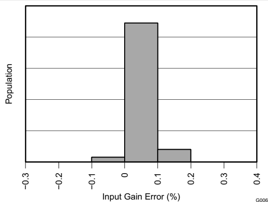
7-5. Shunt Input Gain Error Production Distribution
