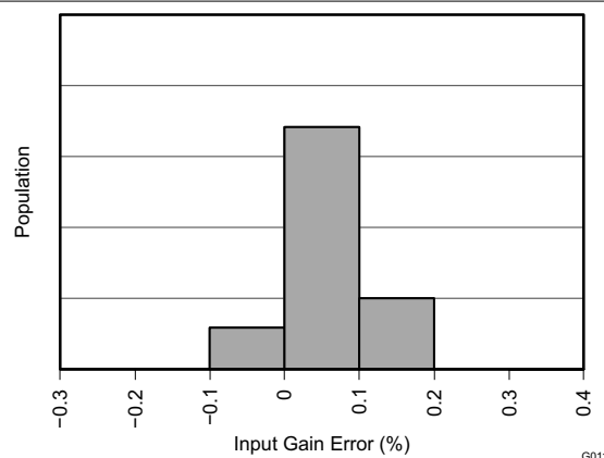
FIG 7-10. Bus Input Gain Error Production Distribution
