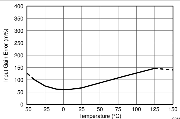
FIG 7-11. Bus Input Gain Error vs. Temperature
