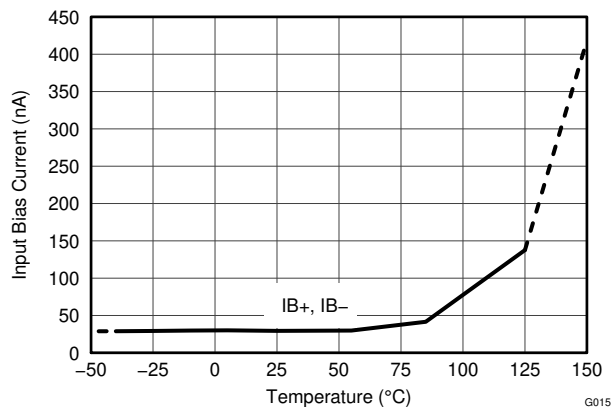
7-14. Input Bias Current vs. Temperature (Shutdown)
