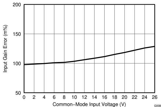
FIG 7-7. Shunt Input Gain Error vs. Common-Mode Voltage
