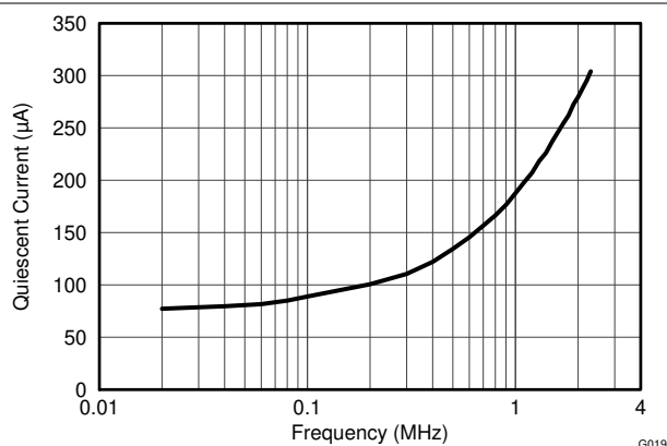
7-18. Shutdown I_Q vs. I^2C Clock Frequency
