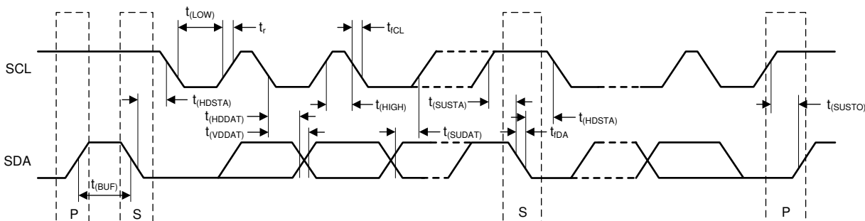
图 8-13. Bus Timing
