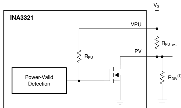
Figure 8-2. Power-Valid Output Structure
