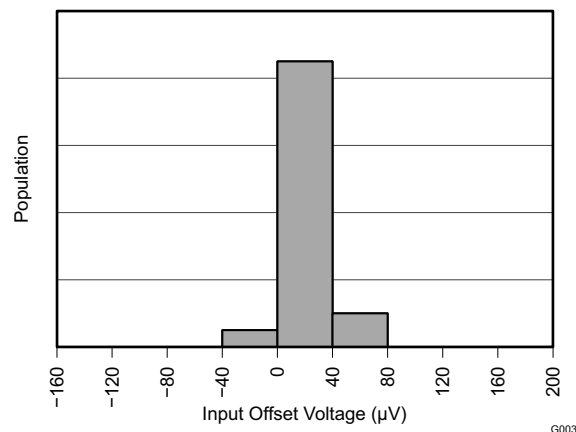
7-2. Shunt Input Offset Voltage Production Distribution
