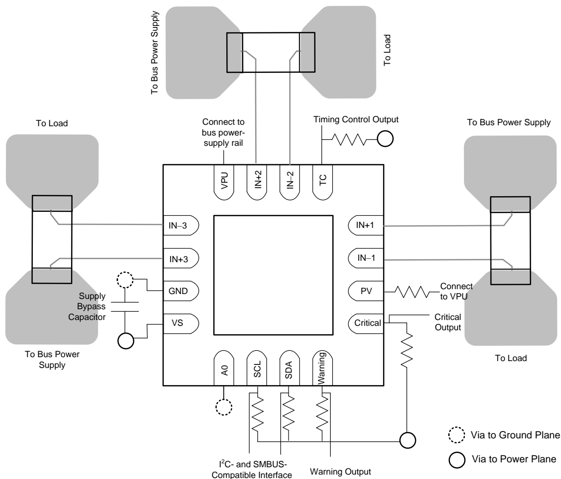
55. Layout Example
