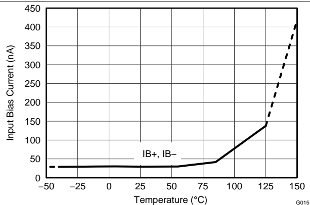
FIG 14. Input Bias Current vs Temperature (Shutdown)
