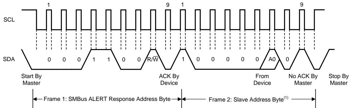
図 30. Timing Diagram for SMBus Alert
