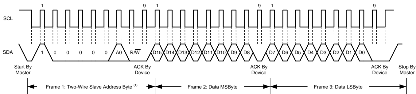
図 28. Timing Diagram for Write Word Format
