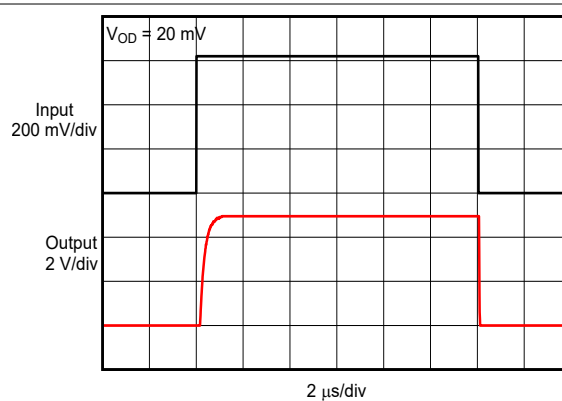
6-40. Comparator Propagation Delay
