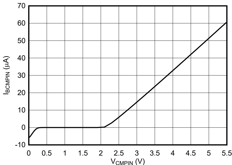
FIG 7-3. Comparator I_{BCMPIN} vs V_{CMPIN}
