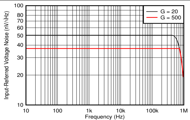
6-24. Input Referred Noise vs Frequency
