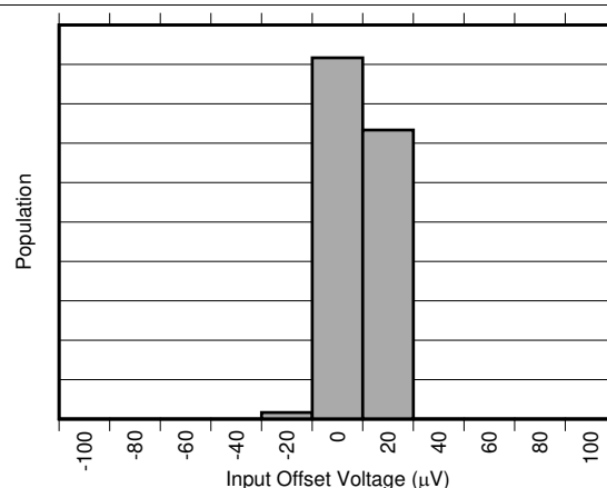
FIG 2. Input Offset Voltage Distribution (INA30xA2)
