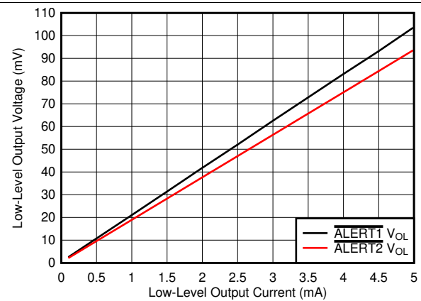
FIG 38. Comparator Alert V_{\text{OL}} vs I_{\text{OL}}
