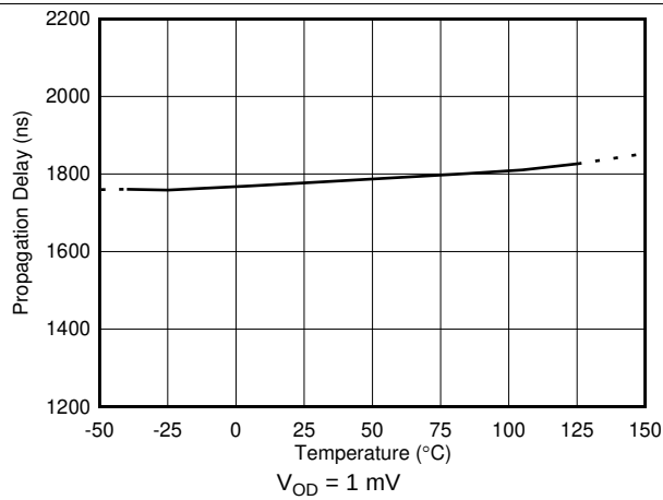
FIG 37. Comparator 2 Propagation Delay vs Temperature
