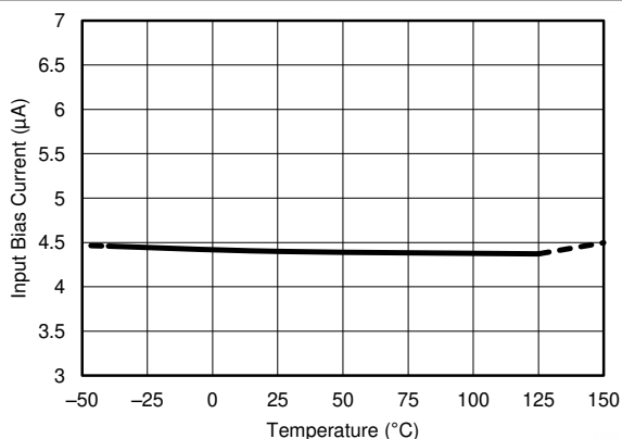
FIG 6-9. Input Bias Current vs. Temperature (Enabled)
