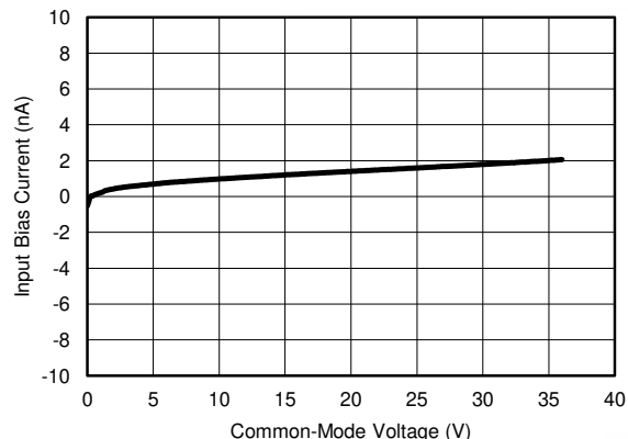
FIG 6-8. Input Bias Current vs. Common-Mode Voltage (Disabled)
