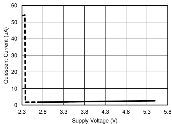
FIG 6-12. Quiescent Current vs. Supply Voltage (Disabled)
