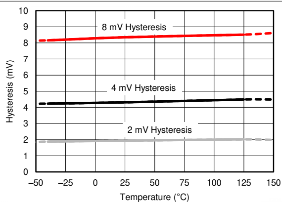
FIG 6-18. Hysteresis vs. Temperature
