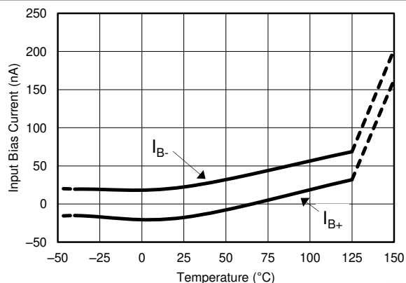
FIG 6-10. Input Bias Current vs. Temperature (Disabled)
