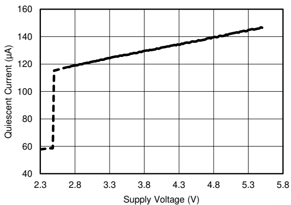
FIG 6-11. Quiescent Current vs. Supply Voltage (Enabled)
