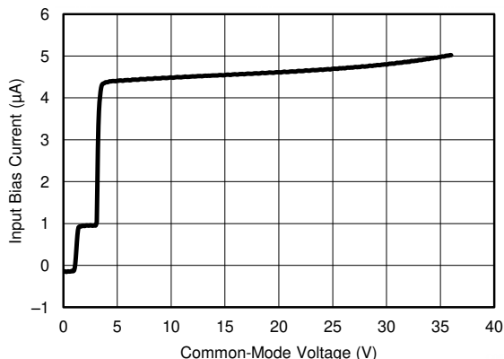
FIG 6-7. Input Bias Current vs. Common-Mode Voltage (Enabled)
