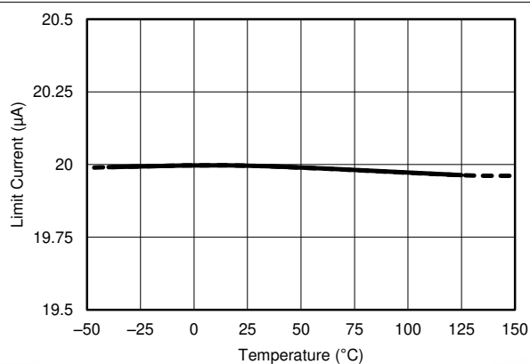
FIG 6-17. Limit Current Source vs. Temperature
