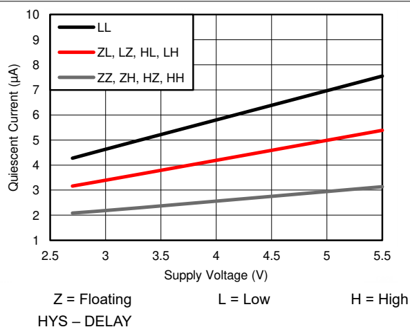
FIG 6-16. Quiescent Current vs. HYS and DELAY Settings (Disabled)
