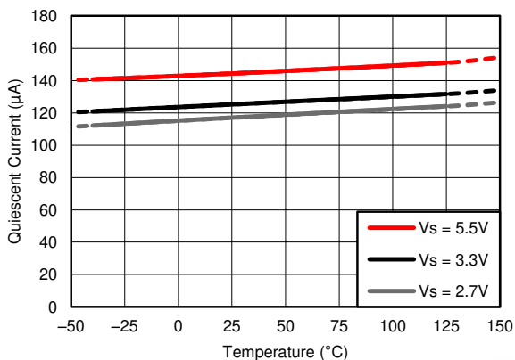
FIG 6-13. Quiescent Current vs. Temperature (Enabled)
