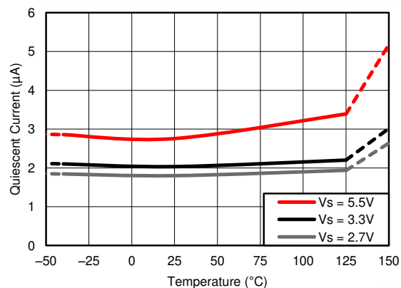
FIG 6-14. Quiescent Current vs. Temperature (Disabled)
