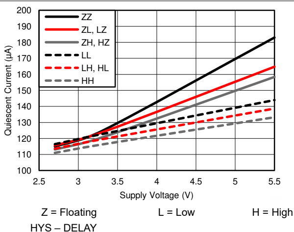
FIG 6-15. Quiescent Current vs. HYS and DELAY Settings (Enabled)
