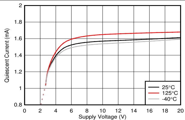
FIG 6-29. Quiescent Current vs Supply Voltage
