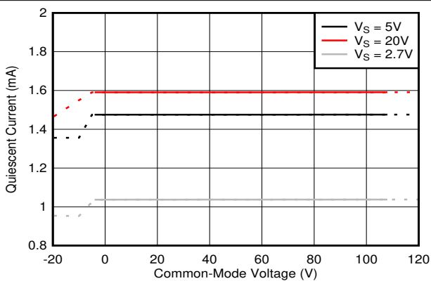
FIG 6-30. Quiescent Current vs Common-Mode Voltage
