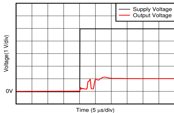
6-33. Start-Up Response
