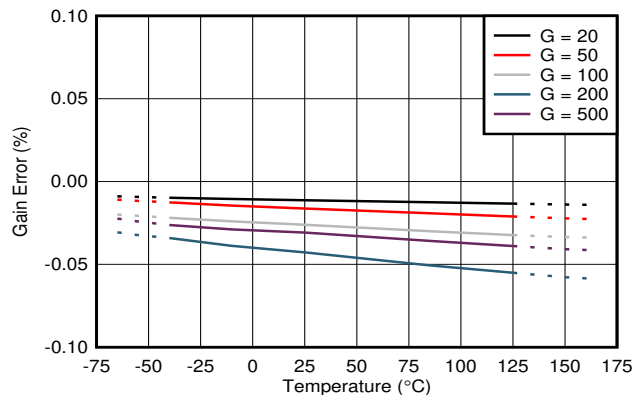
FIG 6-10. Gain Error vs Temperature
