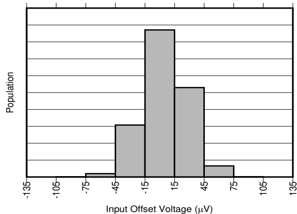
6-1. INA293x1 Input Offset Production Distribution
