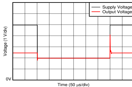
6-34. Supply Transient Response
