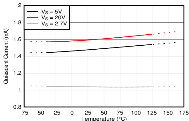
FIG 6-27. Quiescent Current vs Temperature
