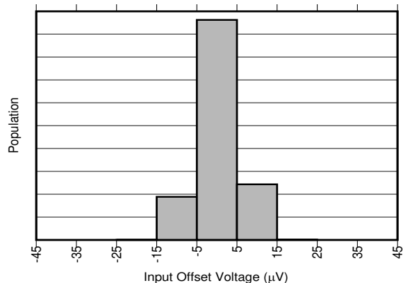
6-3. INA293x3 Input Offset Production Distribution
