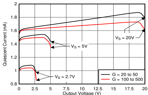
FIG 6-26. Quiescent Current vs Output Voltage
