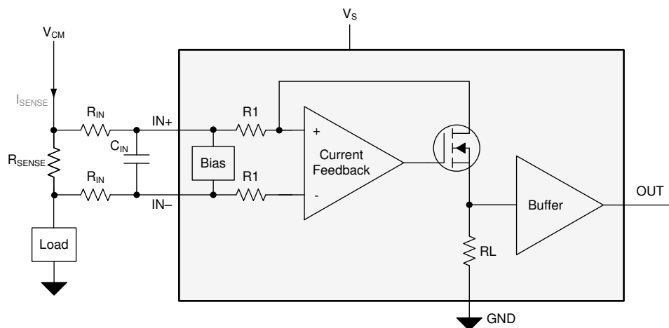
図 8-1. Filter at Input Pins
