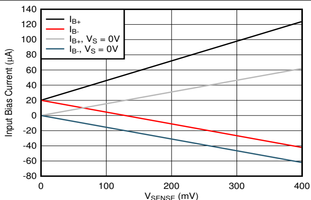
6-16. INA293x2Q, INA293x3Q Input Bias Current vs V_{\text{SENSE}}
