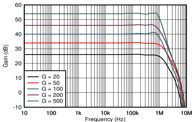
FIG 6-9. Gain vs Frequency
