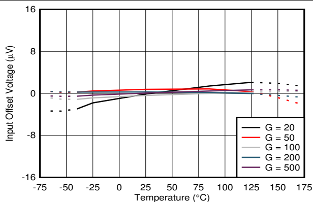
6-6. Input Offset Voltage vs Temperature
