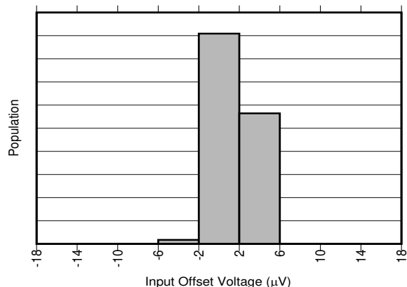
6-5. INA293x5 Input Offset Production Distribution
