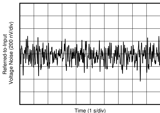
FIG 6-25. Input Referred Noise
