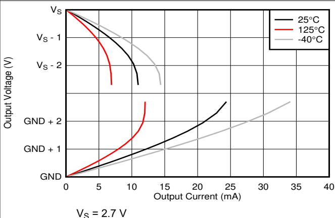
6-18. Output Voltage vs Output Current
