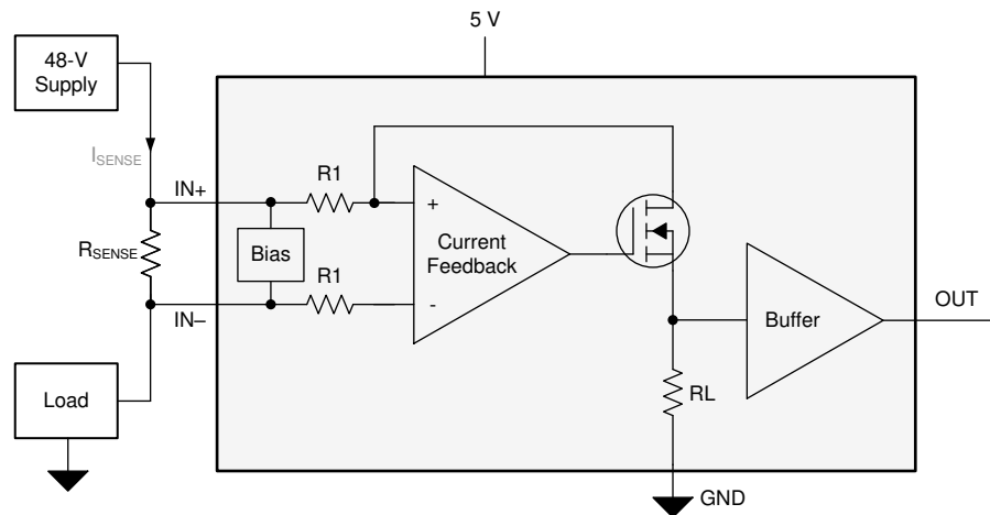
Figure 7-2. Unidirectional Application
