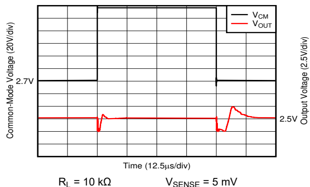
6-23. Common-Mode Voltage Fast Transient Pulse, A5 devices
