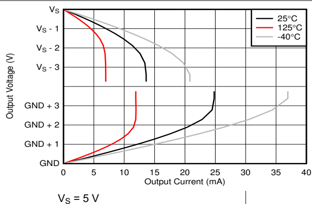
6-11. Output Voltage vs Output Current
