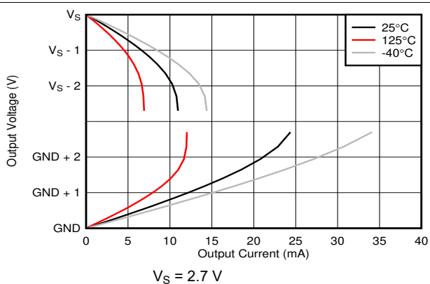
6-10. Output Voltage vs Output Current
