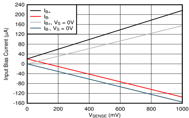
6-7. Input Bias Current vs V_{SENSE} , A1 devices
