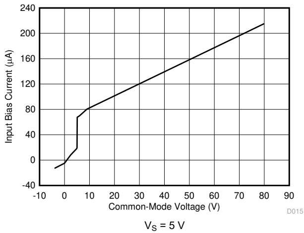
6-15. Input Bias Current vs Common-Mode Voltage
