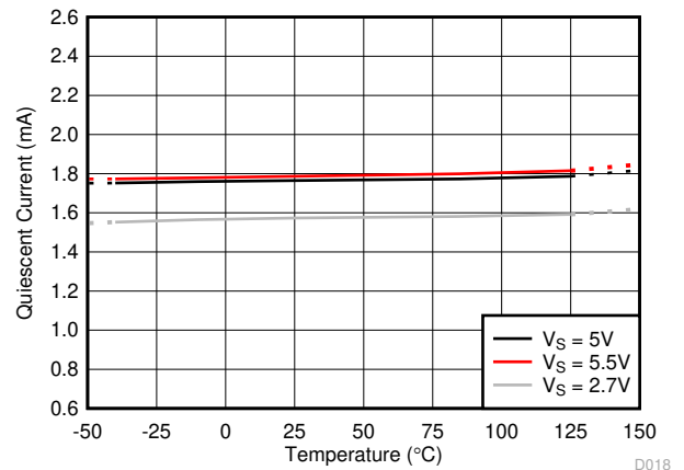
6-18. Quiescent Current vs Temperature
