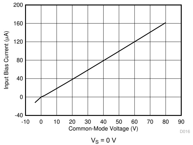
6-16. Input Bias Current vs Common-Mode Voltage
