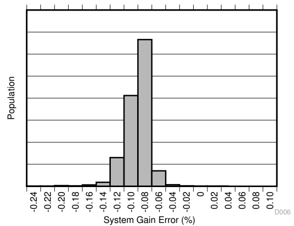
FIG 6-6. Gain Error Production Distribution (INA253A1-Q1)
