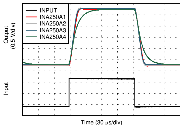
✎ 6-27. Step Response
