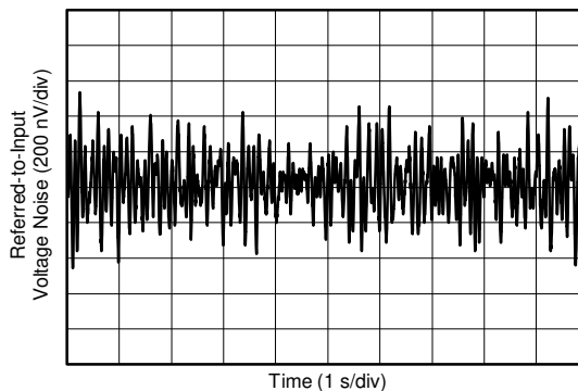
✎ 6-26. 0.1-Hz to 10-Hz Voltage Noise (Referred-to-Input)
