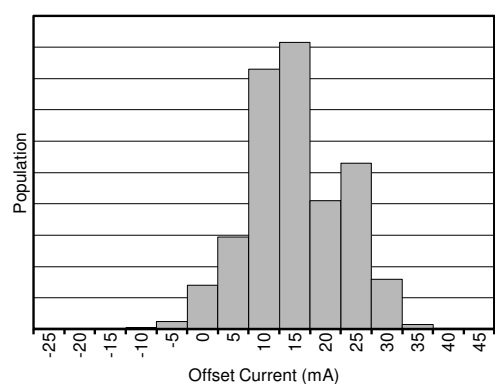
图 6-2. INA250A2 Input Offset Distribution
