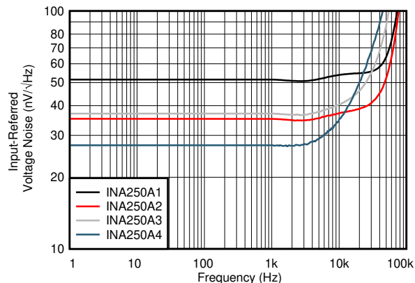
✎ 6-25. Input-Referred Voltage Noise vs Frequency
