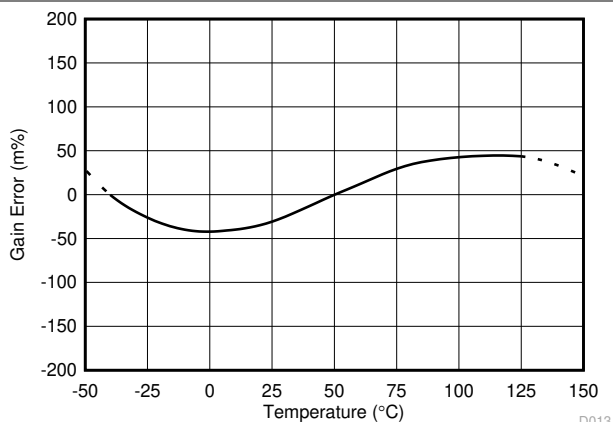
図 5-13. Power Gain Error vs Temperature
