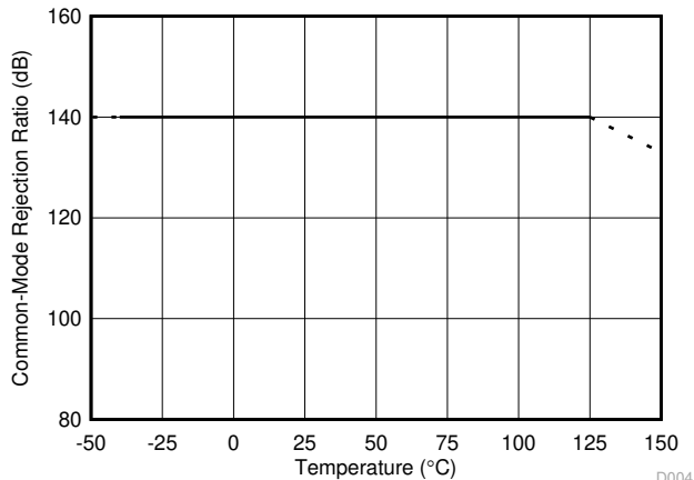
5-4. Shunt Input CMRR vs Temperature
