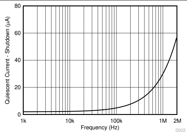
図 5-22. Shutdown I_Q vs SCL Frequency
