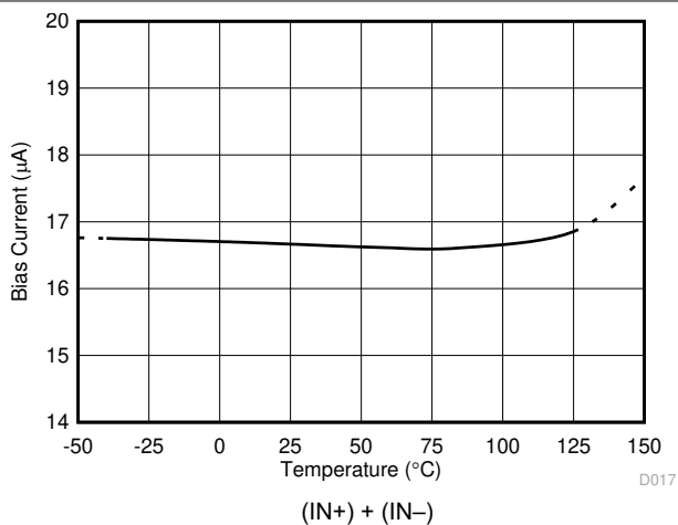
図 5-17. Input Bias Current vs Temperature
