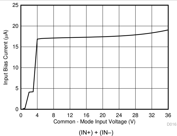
図 5-16. Input Bias Current vs Common-Mode Voltage
