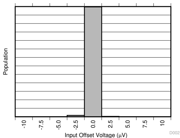
5-2. Shunt Input Offset Voltage Production Distribution
