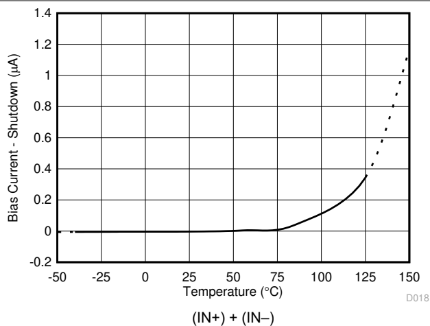
図 5-18. Input Bias Shutdown Current vs Temperature
