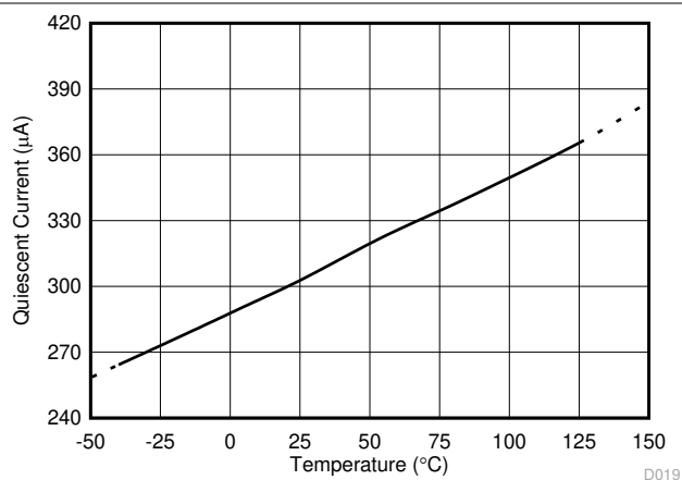
図 5-19. Active I_Q vs Temperature
