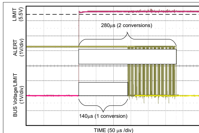
図 7-2. Alert Response ( t_{CT} = 140\mu s)
