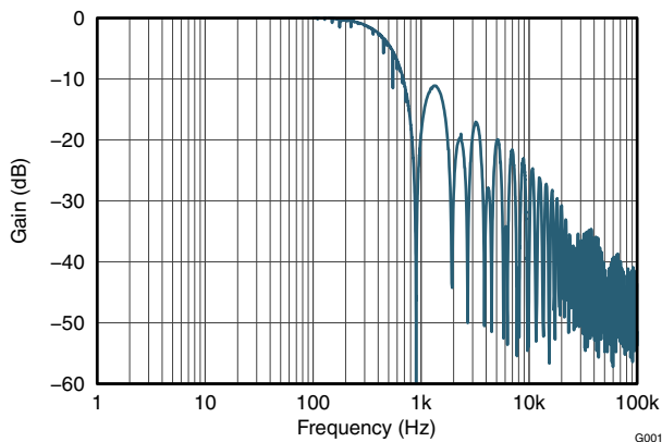
5-1. Frequency Response
