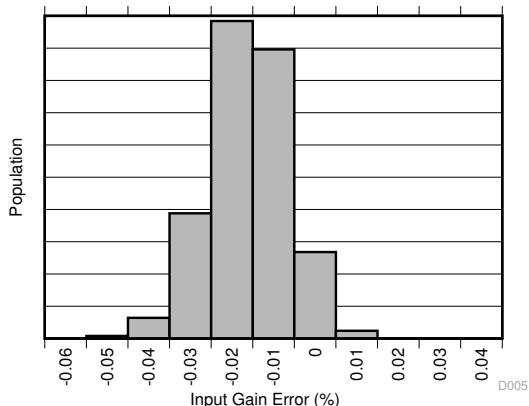
5-5. Shunt Input Gain Error Production Distribution
