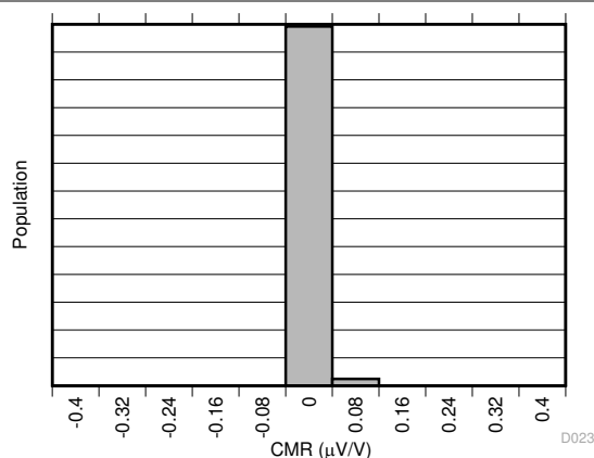
図 5-14. Input Common-Mode Rejection Distribution
