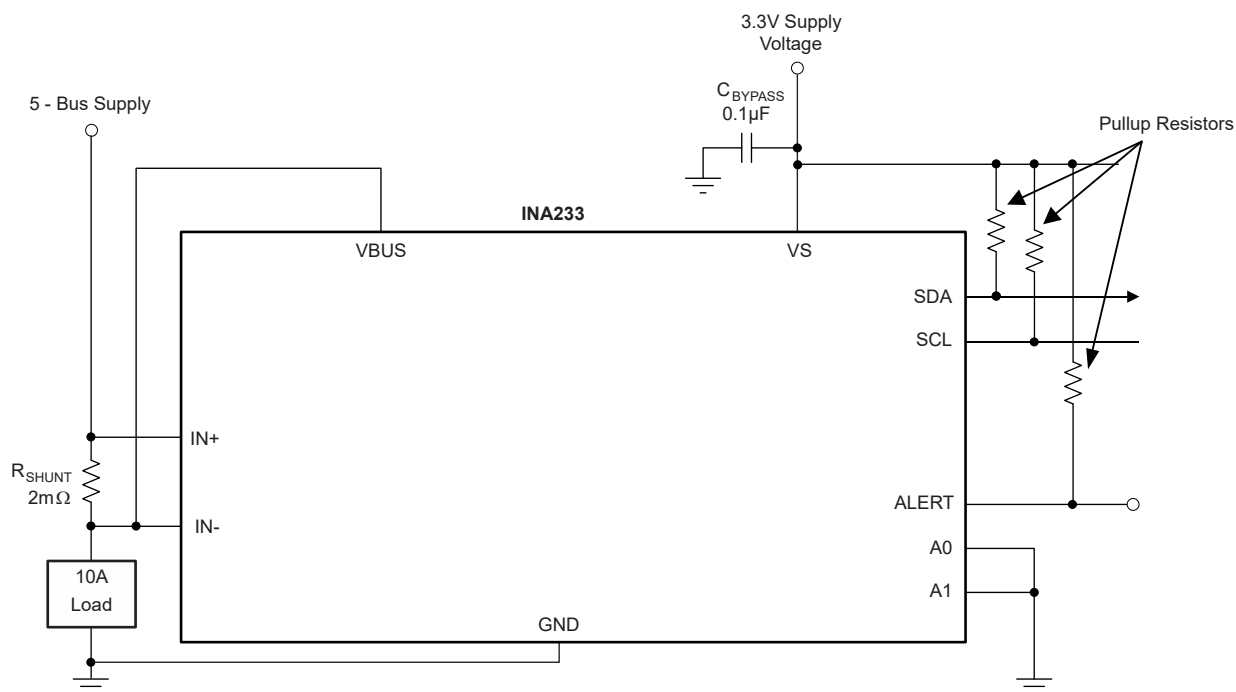
図 7-1. Typical High-Side Sensing Circuit Configuration, INA233
