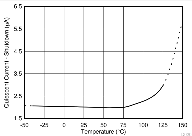
図 5-20. Shutdown I_Q vs Temperature
