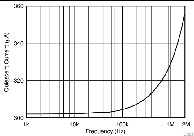
図 5-21. Active I_Q vs SCL Frequency
