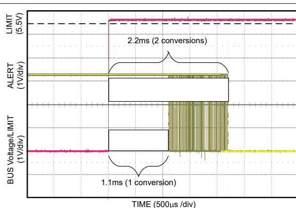
図 7-3. Alert Response ( t_{CT} = 1.1 ms)
