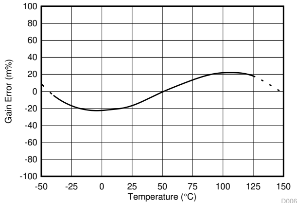
5-6. Shunt Input Gain Error vs Temperature
