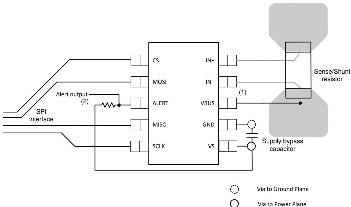
FIG 10-1. INA229-Q1 Layout Example
