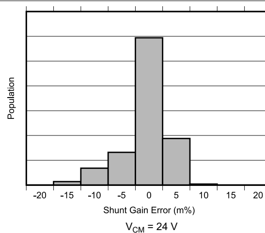
FIG 6-7. Shunt Input Gain Error Production Distribution
