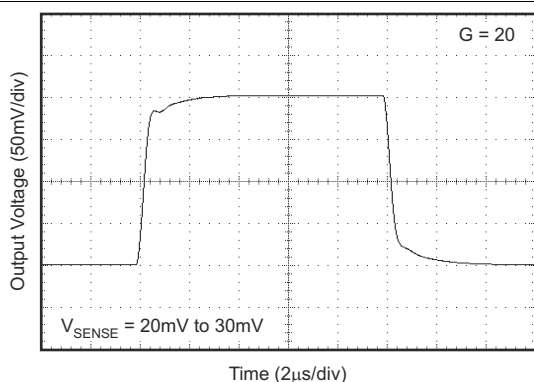
6-12. Step Response
