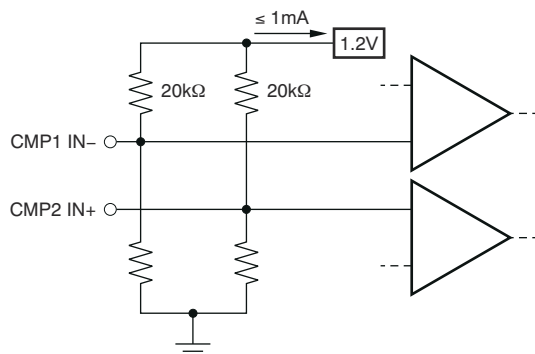
7-6. Limit Current Into Reference \leq 1\text{ mA}
