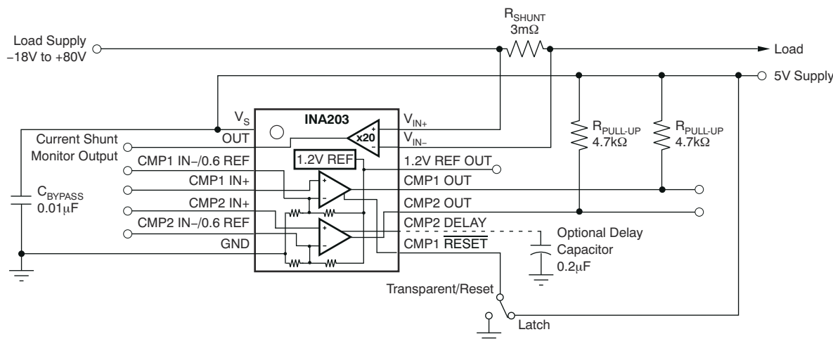
図 7-3. INA20x Basic Connection
