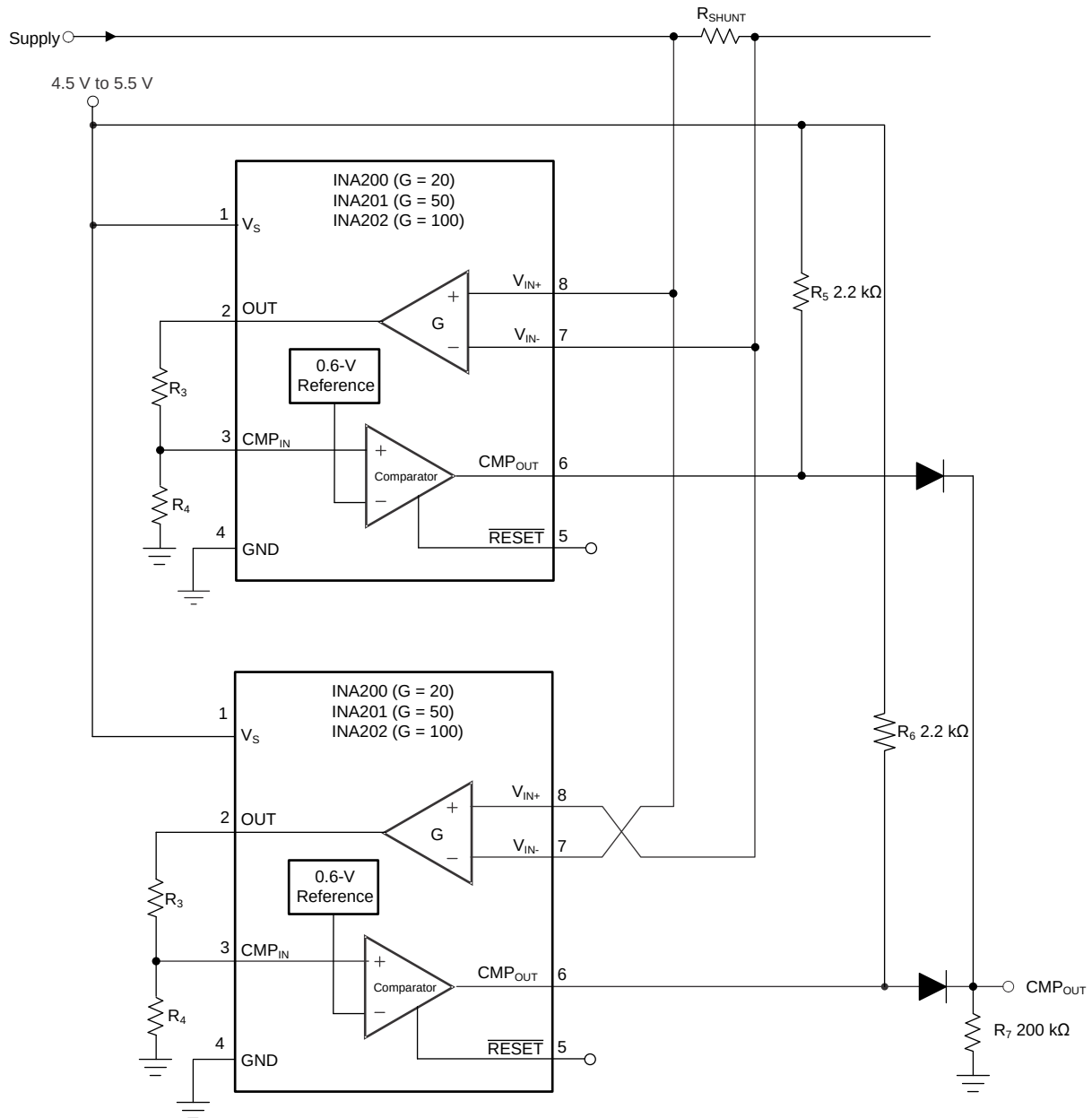
FIG 30. Bidirectional Overcurrent Comparator
