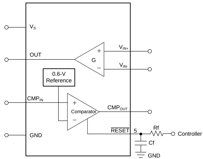
FIG 31. Filter on \overline{RESET} Pin
