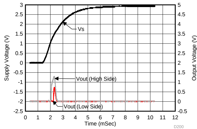
36. Analog Output vs Supply Ramp (INA200)
