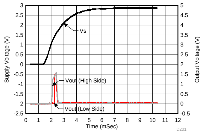
37. Analog Output vs Supply Ramp (INA201)
