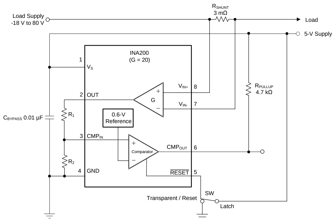
26. INA200 Basic Connections
