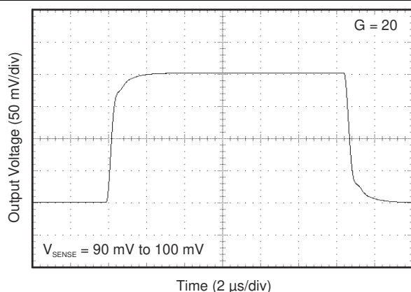
6-15. Step Response
