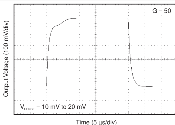
6-16. Step Response
