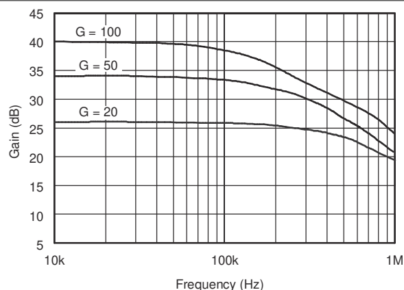
FIG 6-2. Gain vs Frequency
