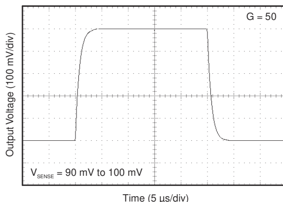
6-18. Step Response
