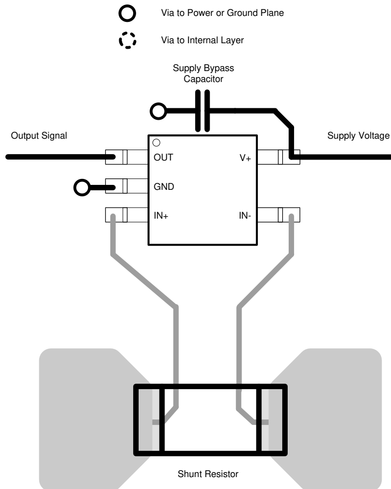
10-1. Recommended Layout
