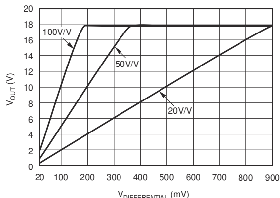
FIG 6-3. Gain Plot
