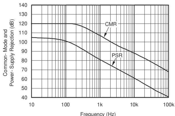
FIG 6-4. Common-Mode and Power-Supply Rejection vs Frequency
