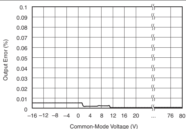
FIG 6-6. Output Error vs Common-Mode Voltage
