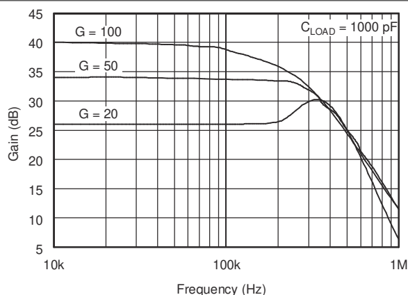
FIG 6-1. Gain vs Frequency
