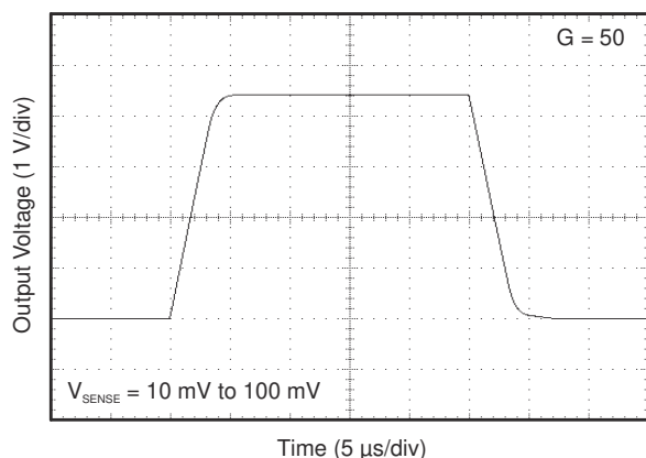
6-17. Step Response
