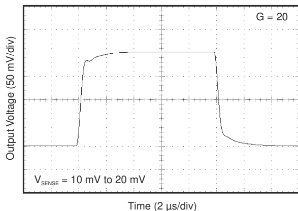
6-13. Step Response
