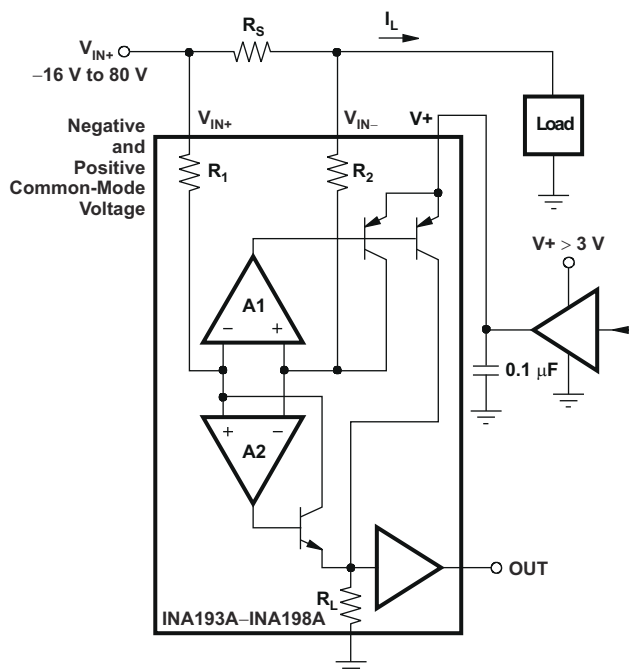
FIG 7-9. INA19xA-Q1 Example Shutdown Circuit
