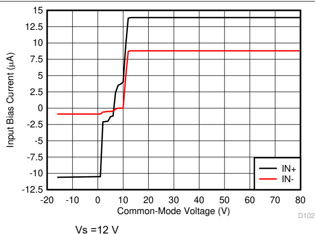
6-10. Input Bias Current vs Common Mode Voltage
