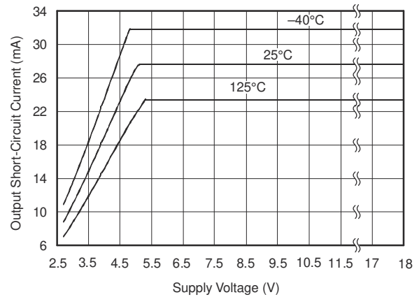
6-12. Output Short Circuit Current vs Supply Voltage
