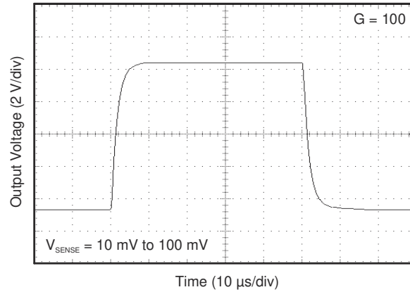
6-19. Step Response
