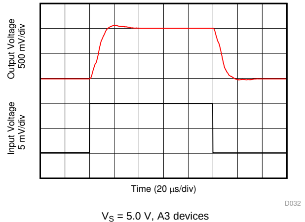
22. Step Response (10-mV PP Input Step)
