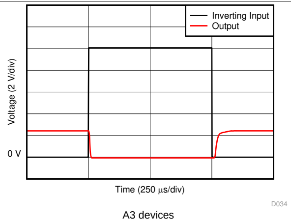
24. Inverting Differential Input Overload
