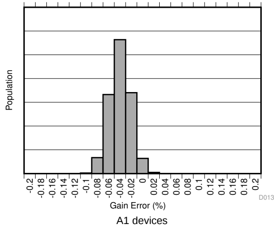
FIG 5. Gain Error Production Distribution
