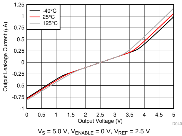
FIG 31. Output Leakage vs Output Voltage (A1, A2, and A3 Devices)
