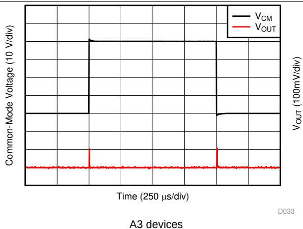
23. Common-Mode Voltage Transient Response
