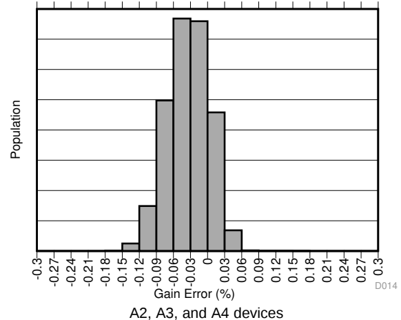
FIG 6. Gain Error Production Distribution
