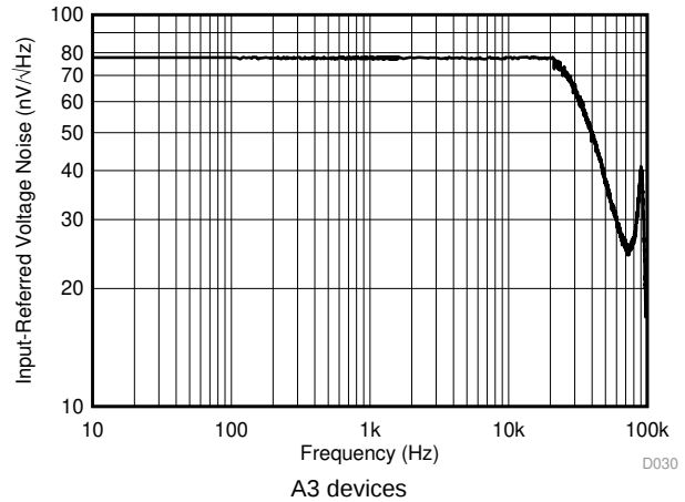
20. Input-Referred Voltage Noise vs Frequency
