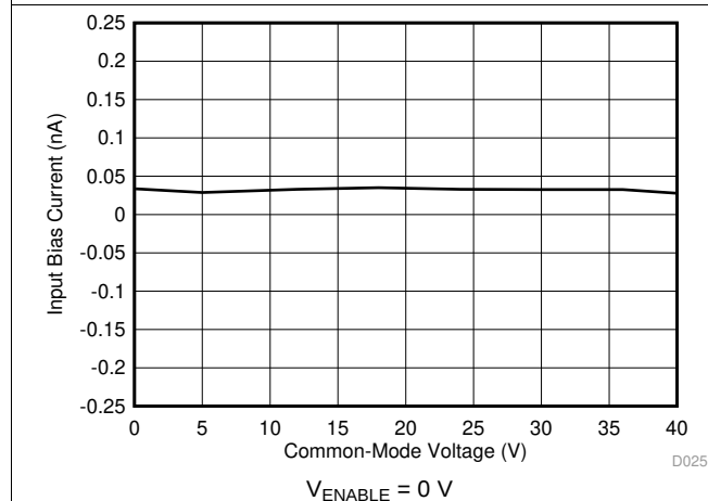
FIG 15. Input Bias Current vs Common-Mode Voltage (Shutdown)
