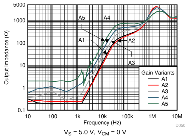
FIG 33. Output Impedance vs Frequency
