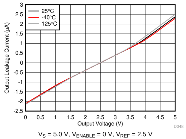
FIG 32. Output Leakage vs Output Voltage (A4 and A5 Devices)
