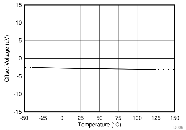
FIG 2. Offset Voltage vs Temperature
