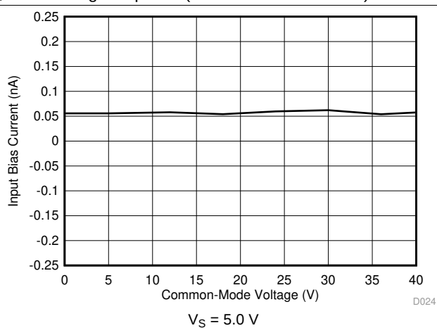
FIG 14. Input Bias Current vs Common-Mode Voltage
