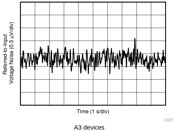
21. 0.1-Hz to 10-Hz Voltage Noise (Referred-To-Input)
