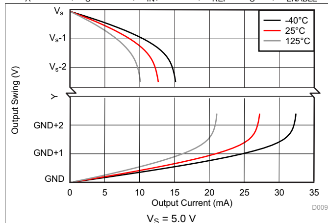
FIG 13. Output Voltage Swing vs Output Current
