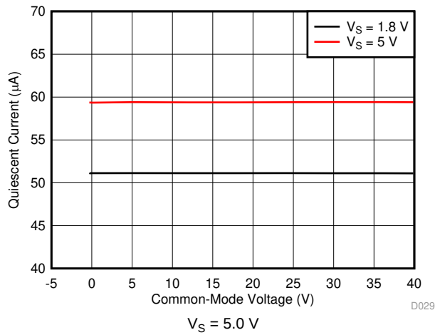
19. Quiescent Current vs Common Mode Voltage
