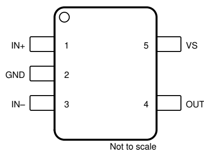
図 6-2. INA180-Q1: DBV Package 5-Pin SOT-23 (Pinout B) Top View
