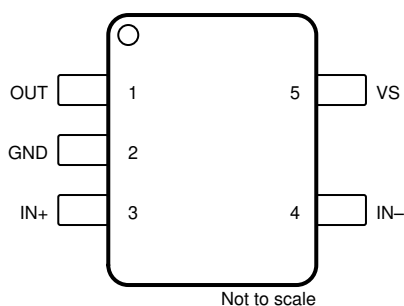
図 6-1. INA180-Q1: DBV Package 5-Pin SOT-23 (Pinout A) Top View
