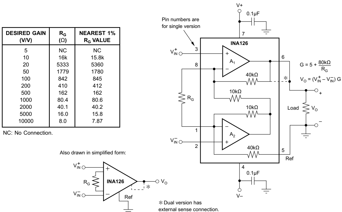
☒ 8-1. Basic Connections
