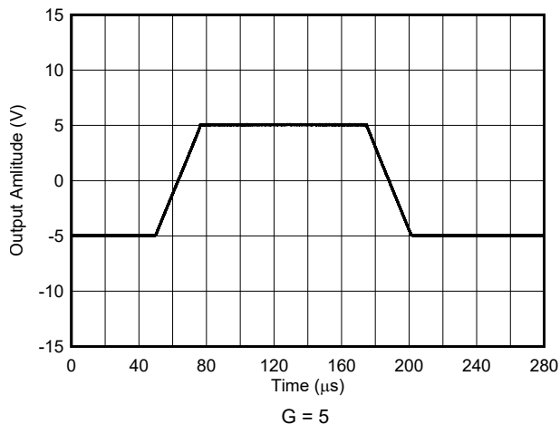
6-16. Large-Signal Response
