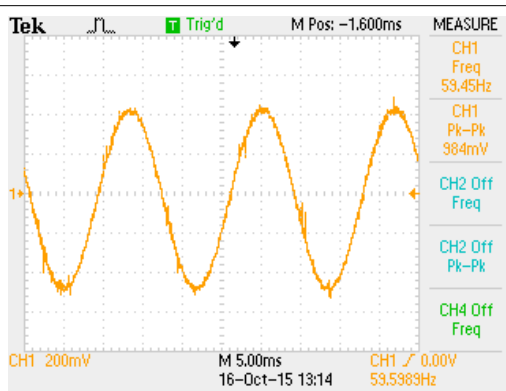
8-4. Common-mode Signal at INA126 Input
