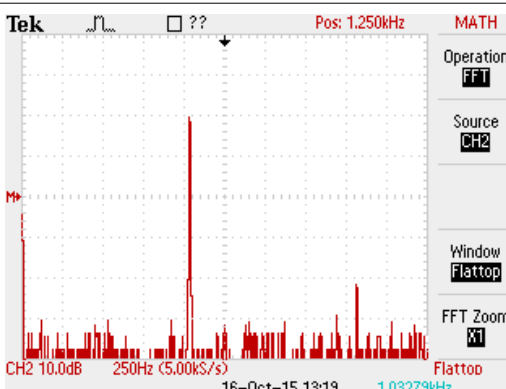
8-7. FFT of the INA126 Output Shows that the 60-Hz Common-mode Signal is Rejected
