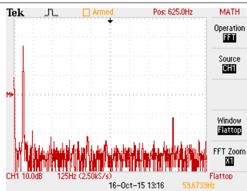
8-5. FFT of Signal in Previous Figure Shows Both the 60-Hz Common-mode Along With 5-kHz Differential Signal
