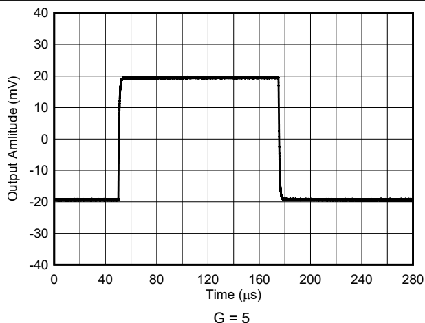
6-14. Small-Signal Response
