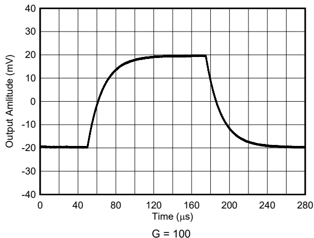
6-15. Small-Signal Response
