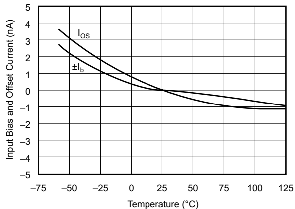
FIG 7-14. Input Bias and Offset Current vs Temperature
