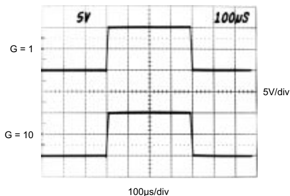
Figure 7-23. Large-Signal Response
