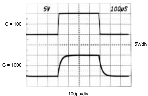
Figure 7-22. Small-Signal Response
