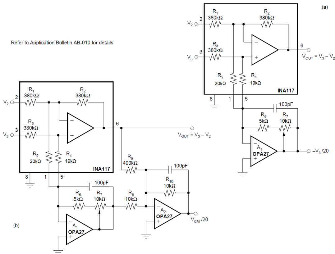
図 7-11. Common-mode Voltage Monitoring
