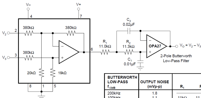
図 7-8. Leakage Current Measurement Circuit
