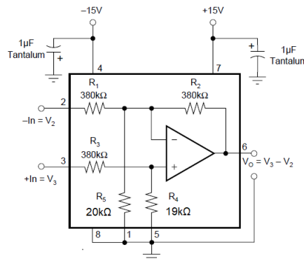
図 7-1. Basic Power and Signal Connections
