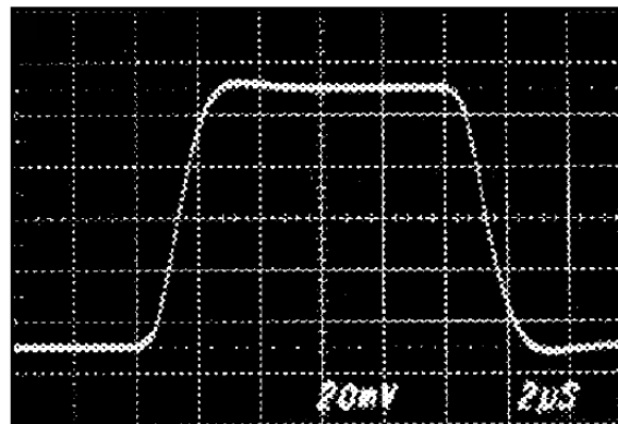
Figure 6-6. Small Signal Step Response C_L = 1000\text{pF}
