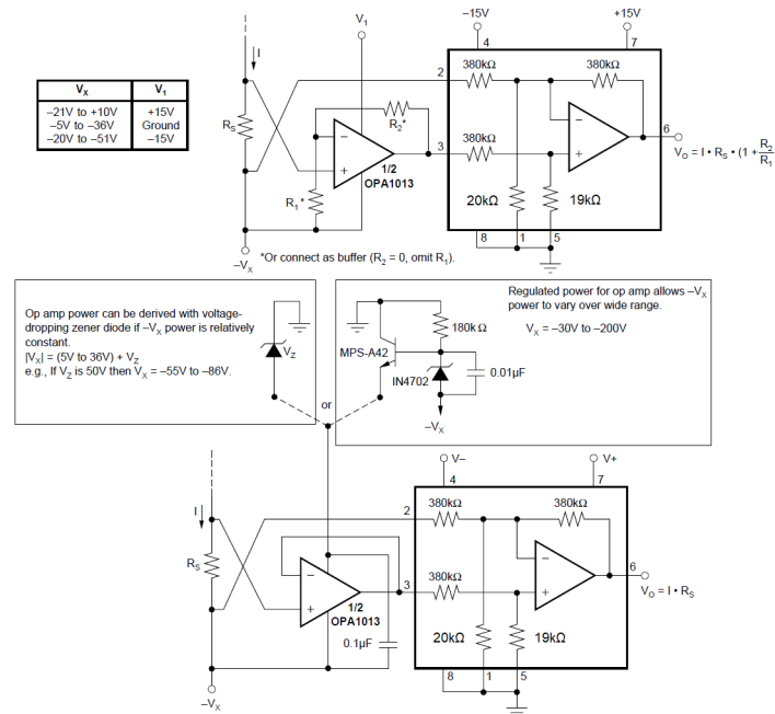
7-7. Current Sensing With Input Buffer
