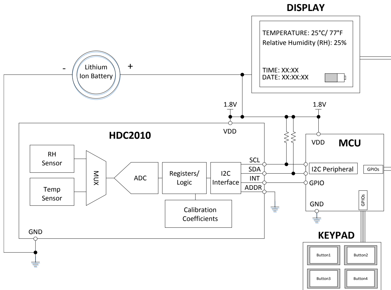
図 9-1. Typical Application Schematic HVAC
