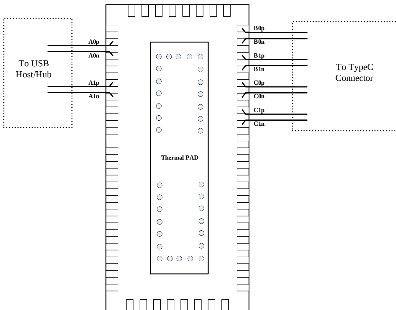
Figure 5. Layout
