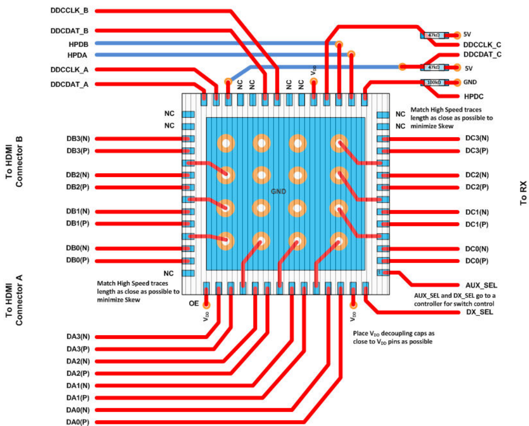
10-3. RTQ Layout for 2:1 HDMI Sink Application
