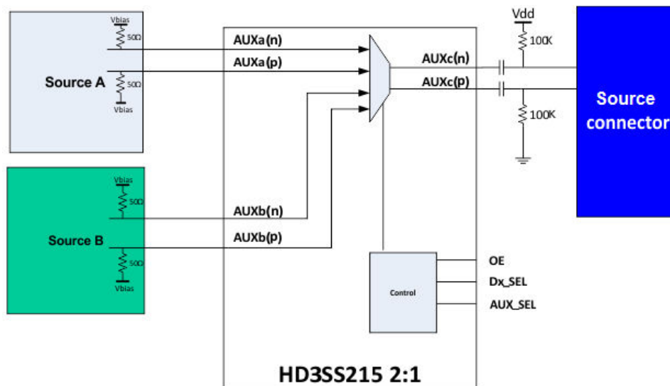
図 9-2. HD3SS215 AUX Channel in 2:1 DisplayPort Application
