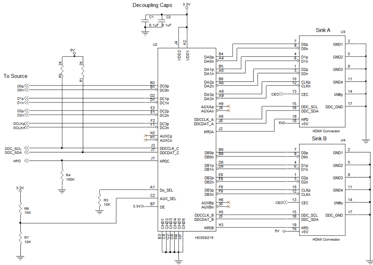
图 9-4. Application Diagram for a 1:2 Configuration with HDMI Source and Connectors
