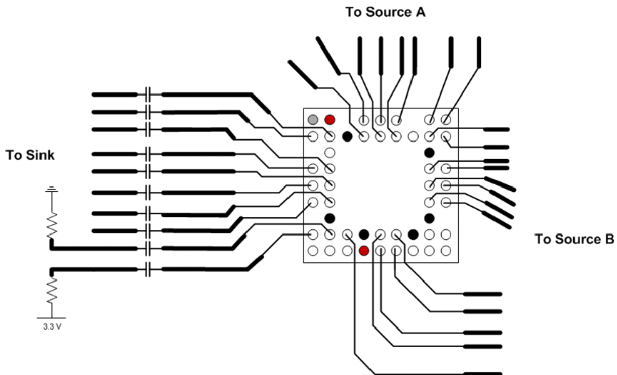
FIG 10-1. Top Layer Layout View
