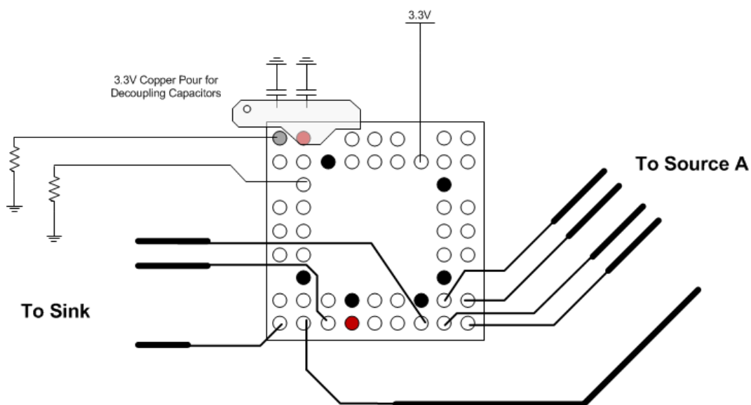
FIG 10-2. Bottom Layer Layout View
