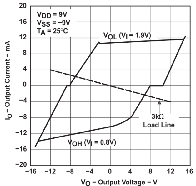
図 5-2. Output Current vs Output Voltage
