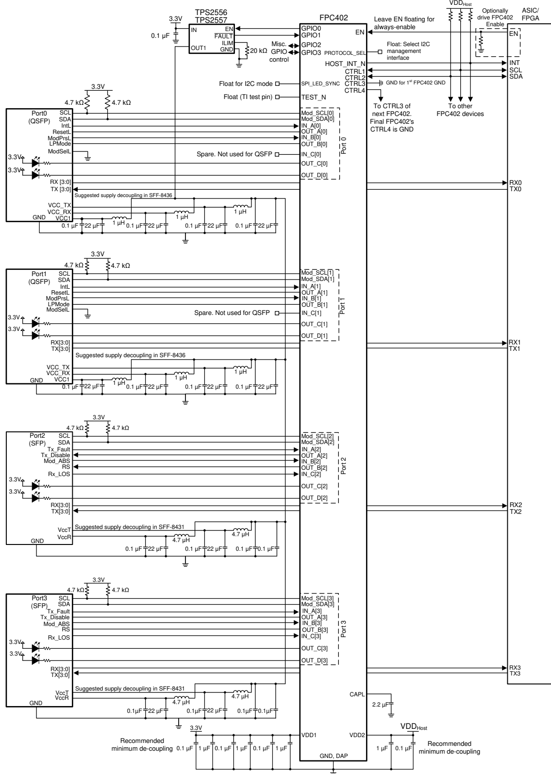
9-3. SFP/QSFP Application Schematic
