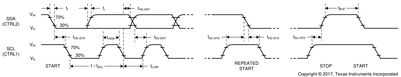
図 8-5. I2C Timing Diagram
