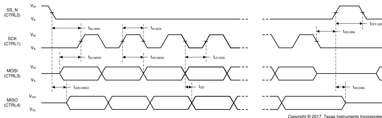
FIG 8-9. SPI Timing Diagram
