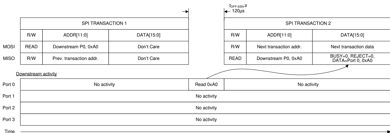
FIG 8-10. SPI Read Consisting of Two Separate SPI Transactions
