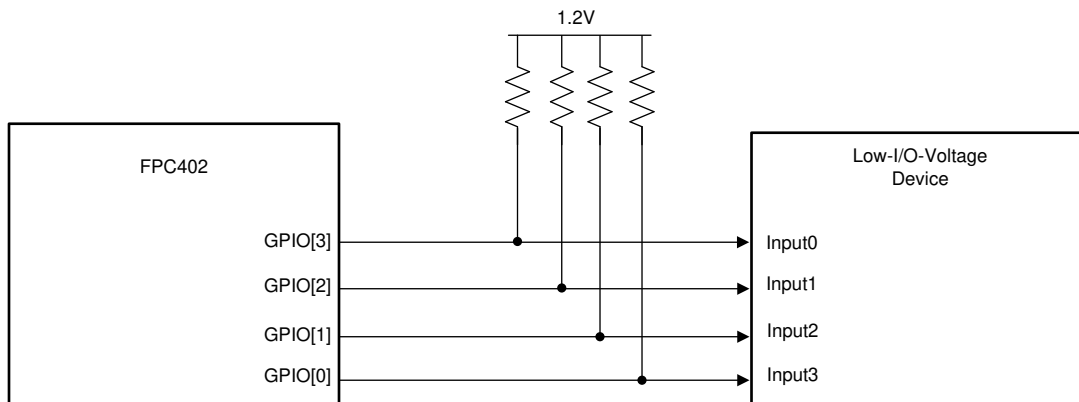
Figure 8-3. Example Use Of External Pullups to Drive Low-I/O-Voltage Devices From GPIOs
