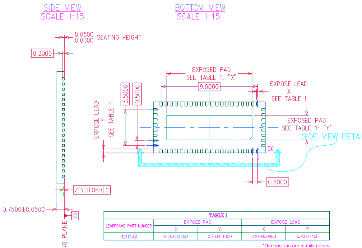
Figure 11-2. Recommended Package Footprint
