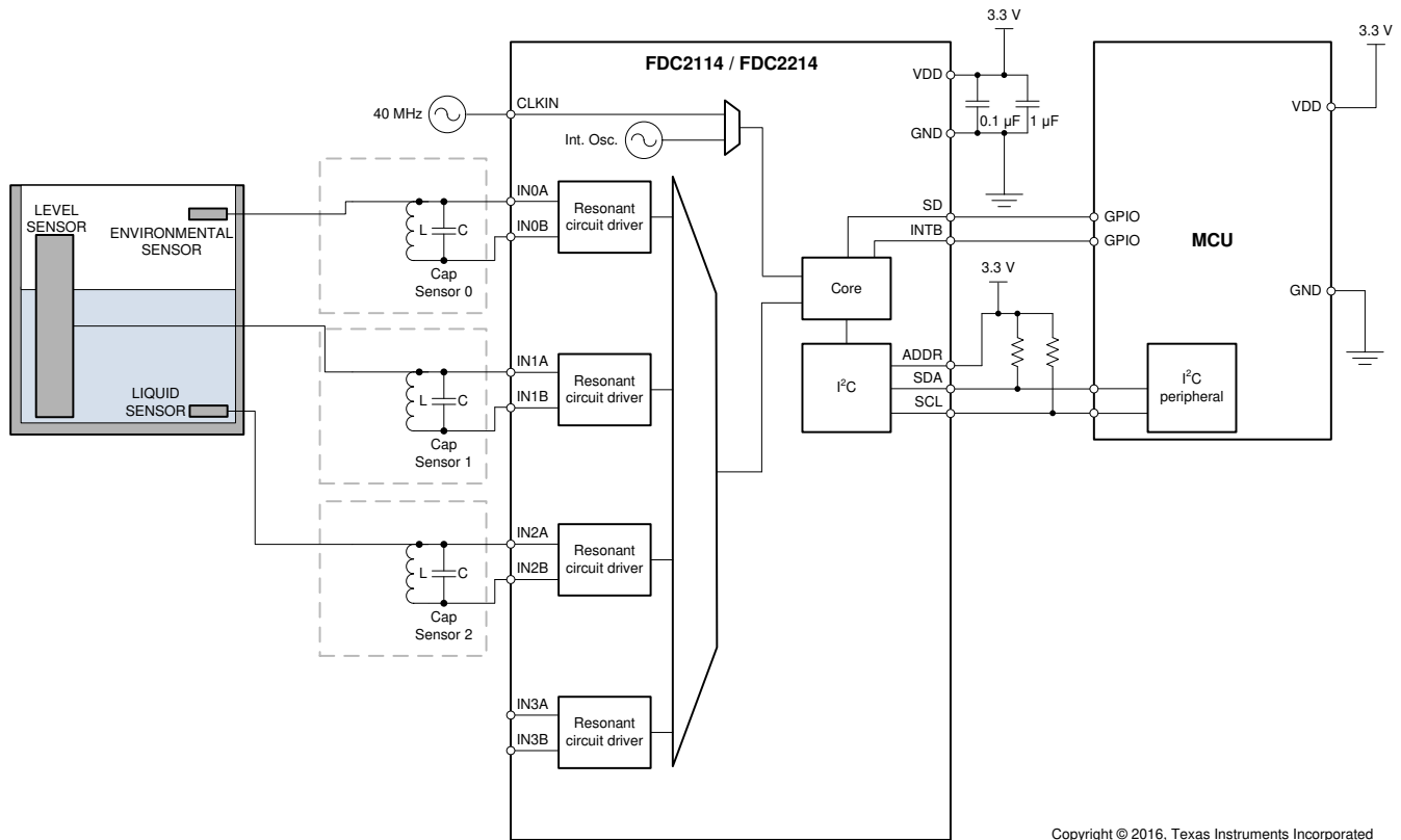
図 7-7. FDC (Liquid Level Measurement)
