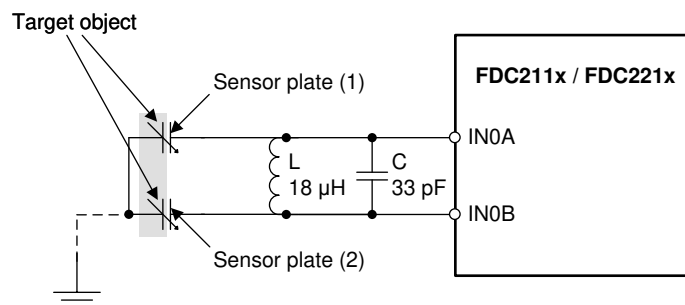
図 7-2. Differential Sensor Configuration
