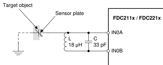
図 7-1. Single-Ended Sensor Configuration
