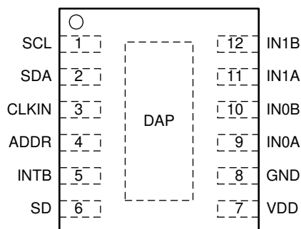
図 4-1. FDC2112/FDC2212 DNT Package 12-Pin WSON Top View
