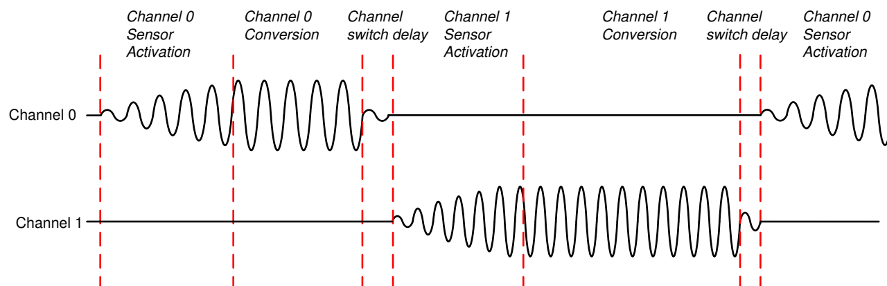
図 6-4. Multi-Channel Mode Sequencing
