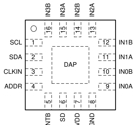
図 4-2. FDC2114/FDC2214 RGH Package 16-Pin WQFN Top View
