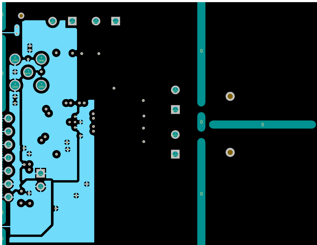
図 7-11. Example PCB Layout: Mid-Layer 2 (Power)
