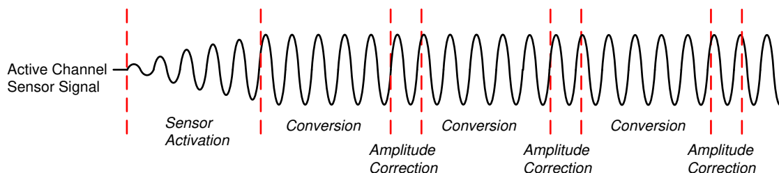
図 6-5. Single-Channel Mode Sequencing
