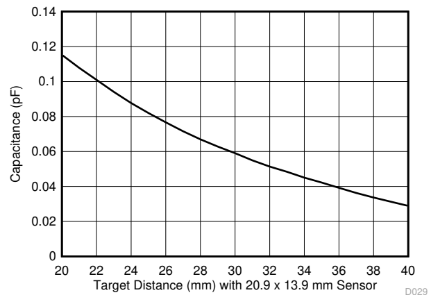
Figure 7-5. FDC2112 / FDC2114: Capacitance vs Target Distance (20mm to 40mm)
