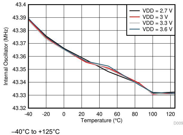
図 5-8. Internal Oscillator Frequency vs Temperature
