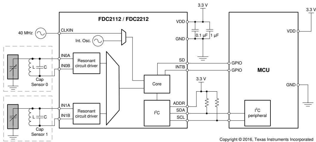
FIG 6-1. Block Diagram for the FDC2112 and FDC2212
