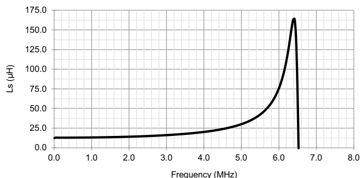
図 7-3. Example Coil Inductance vs Frequency
