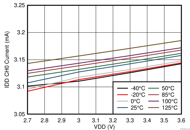
Figure 5-3. Active Mode I_{DD} vs V_{DD}
