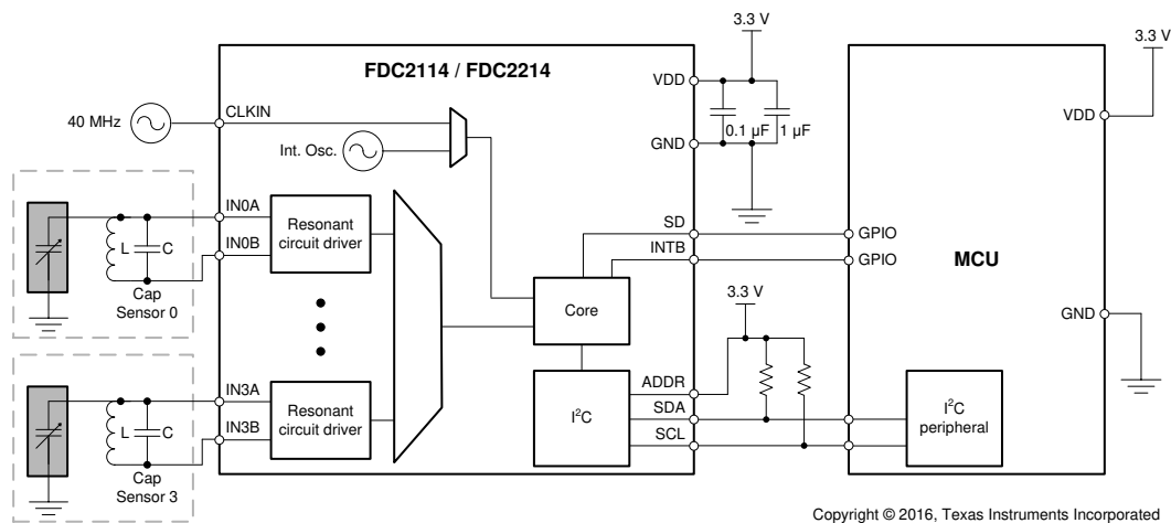
FIG 6-2. Block Diagram for the FDC2114 and FDC2214
