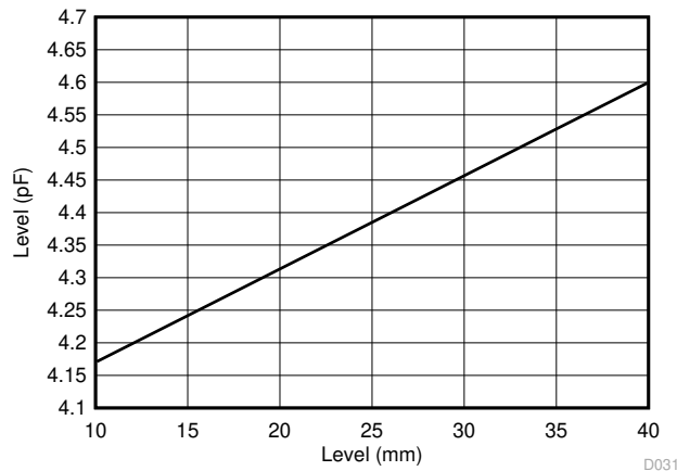
7-8. Electrode Capacitance vs Liquid Level
