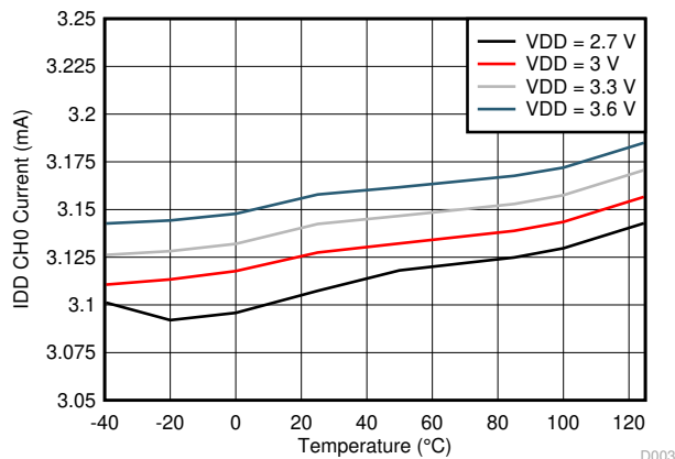
Figure 5-2. Active Mode I_{DD} vs Temperature
