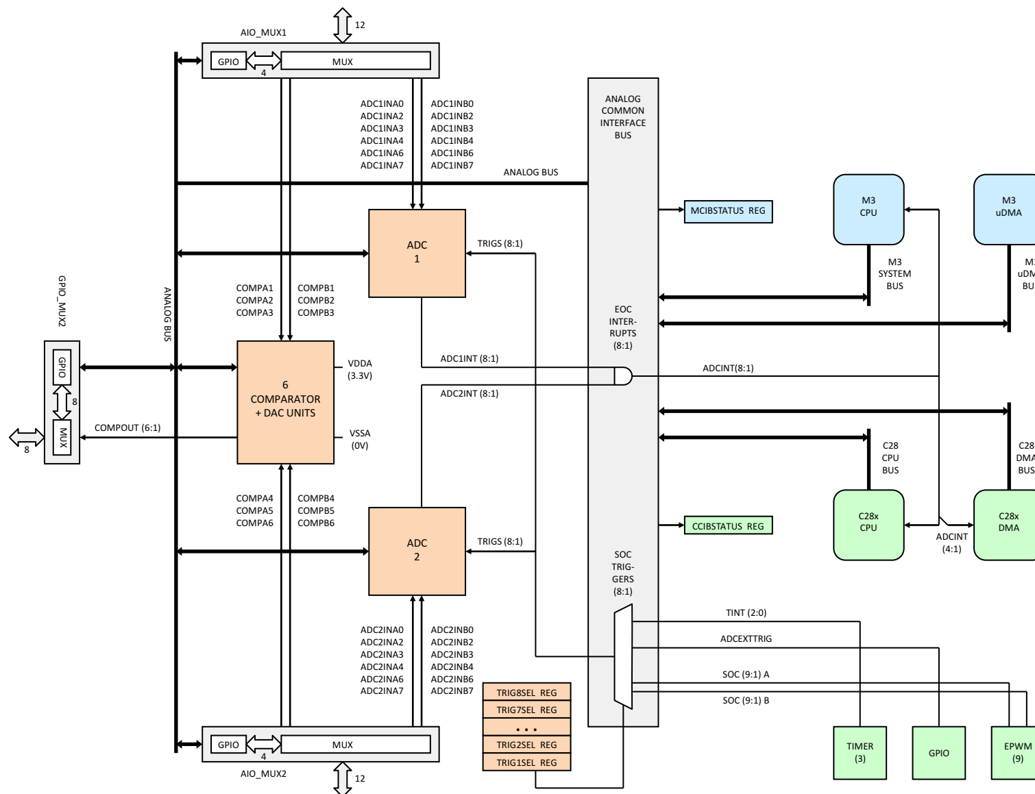
Figure 6-3. Analog Subsystem
