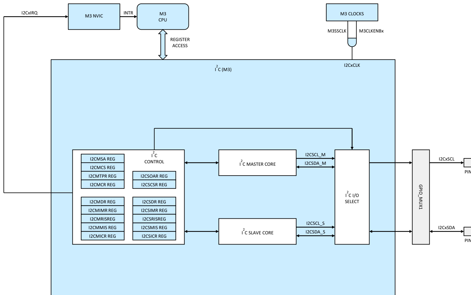
Figure 5-32. I2C (Cortex-M3)
