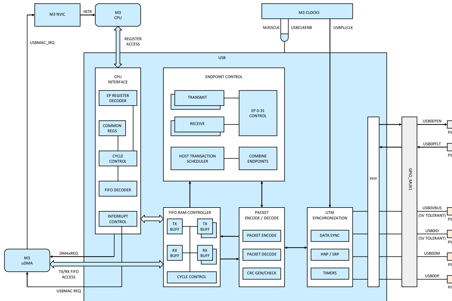
Figure 5-34. USB
