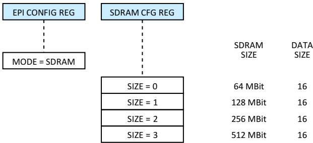
Figure 5-18. EPI SDRAM Mode
