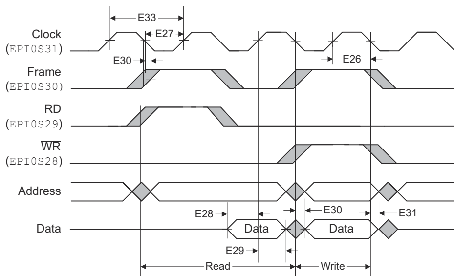
7-28. General-Purpose Mode Read and Write Timing
