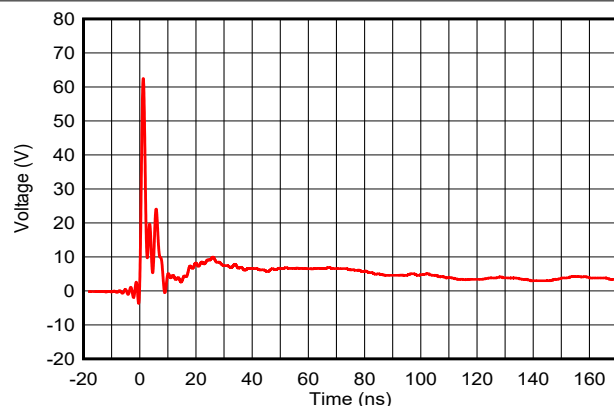
図 5-1. +8kV IEC 61000-4-2 Clamping Voltage Waveform
