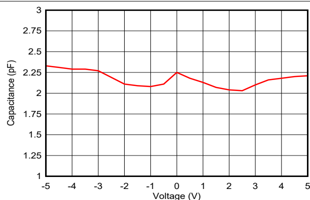
図 5-3. Capacitance vs. Bias Voltage
