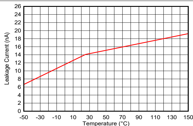
図 5-5. Leakage Current vs. Temperature
