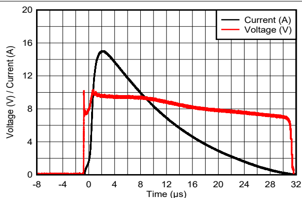
図 5-4. 8/20μs Surge Response
