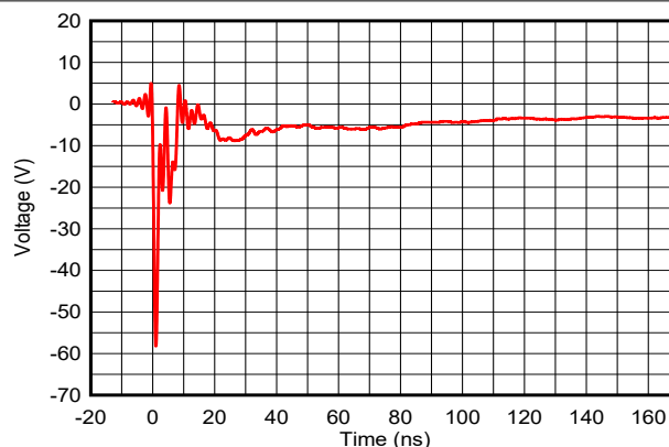
図 5-2. -8kV IEC 61000-4-2 Clamping Voltage Waveform
